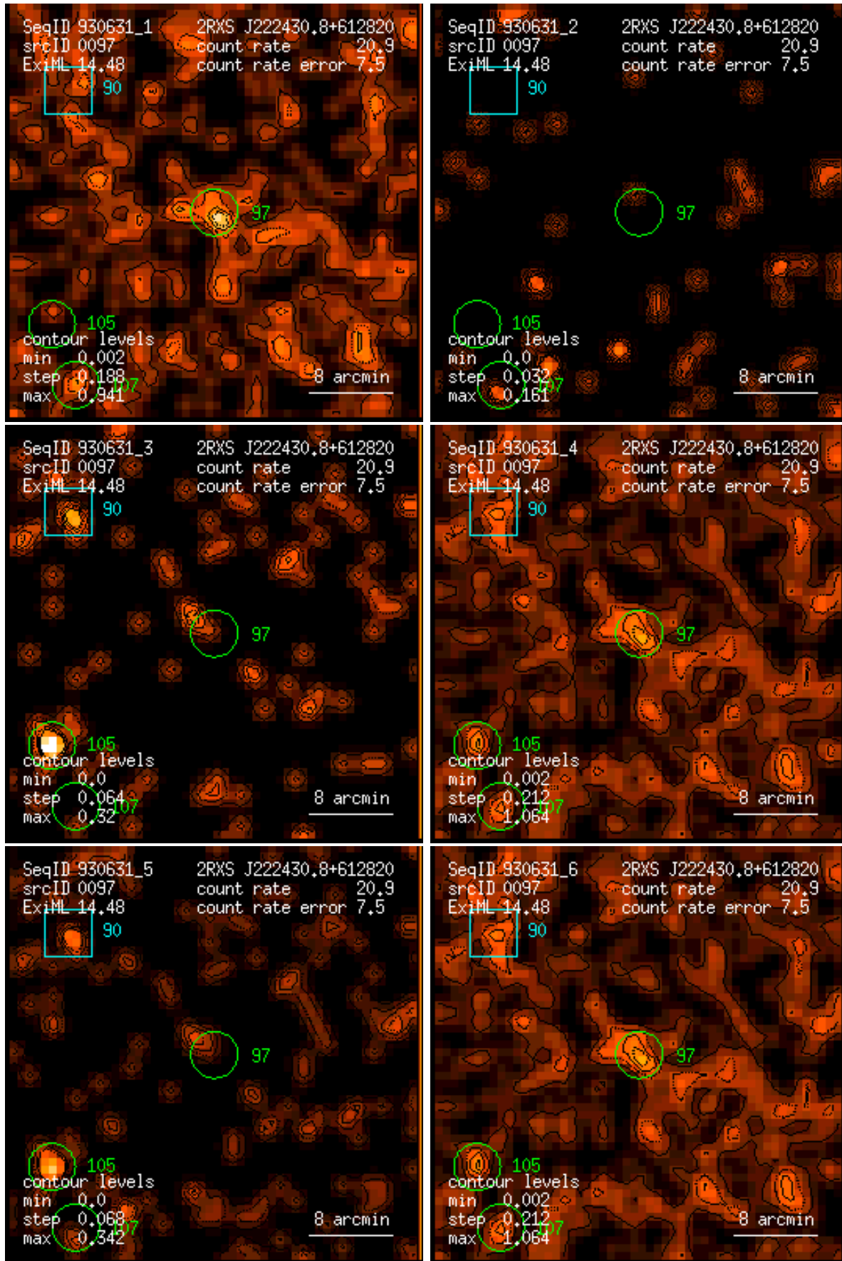
Figure 97: RASS 930631: detection 0097: band rate images, Gaussian filter: (1) PSPC channels 11 – 41, (2) 52 – 90, (3) 91 – 201, (4) 11 – 235, (5) 52 – 201, (6) 11 – 201. Broad band rates in counts/ks. Band rate contour levels in counts/ks/arcmin 2 .
