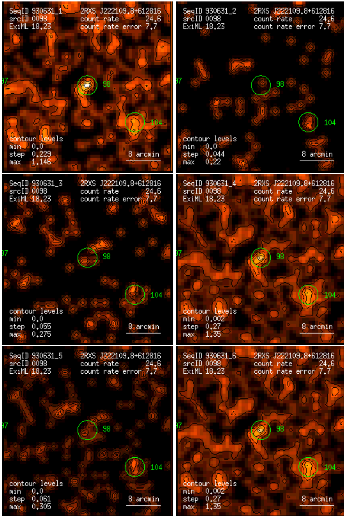
Figure 98: RASS 930631: detection 0098: band rate images, Gaussian filter: (1) PSPC channels 11 – 41, (2) 52 – 90, (3) 91 – 201, (4) 11 – 235, (5) 52 – 201, (6) 11 – 201. Broad band rates in counts/ks. Band rate contour levels in counts/ks/arcmin 2 .
