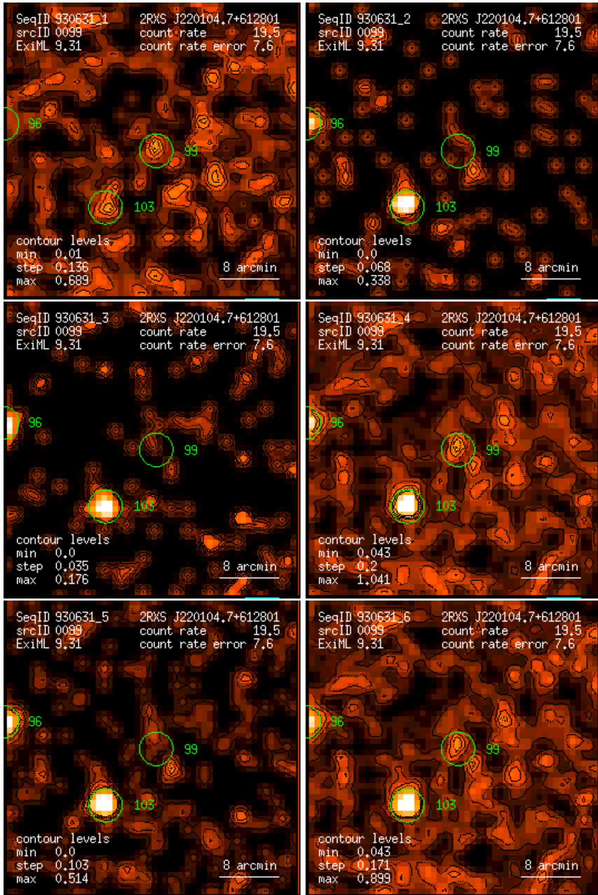
Figure 99: RASS 930631: detection 0099: band rate images, Gaussian filter: (1) PSPC channels 11 – 41, (2) 52 – 90, (3) 91 – 201, (4) 11 – 235, (5) 52 – 201, (6) 11 – 201. Broad band rates in counts/ks. Band rate contour levels in counts/ks/arcmin 2 .
