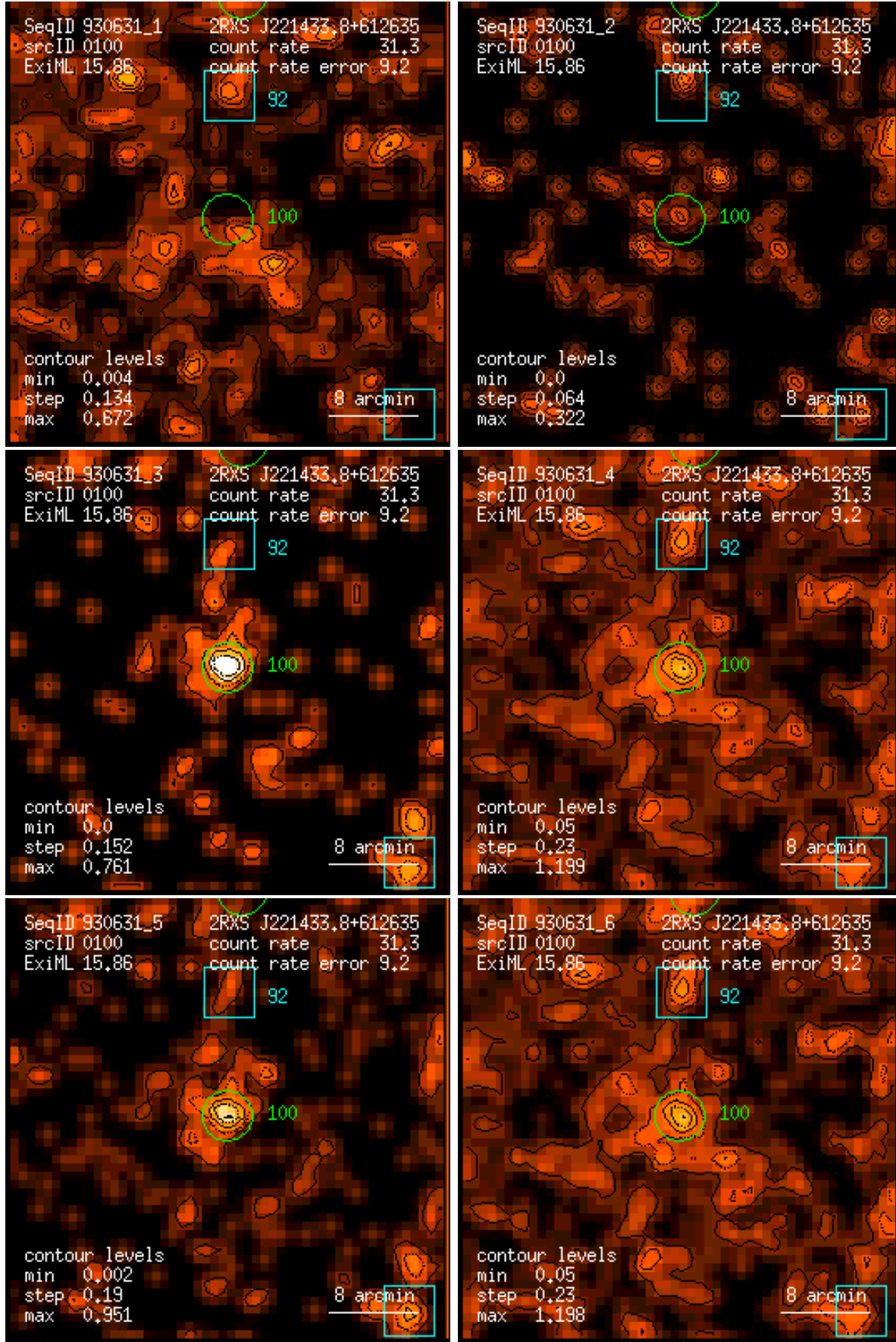
Figure 100: RASS 930631: detection 0100: band rate images, Gaussian filter: (1) PSPC channels 11 – 41, (2) 52 – 90, (3) 91 – 201, (4) 11 – 235, (5) 52 – 201, (6) 11 – 201. Broad band rates in counts/ks. Band rate contour levels in counts/ks/arcmin 2 .
