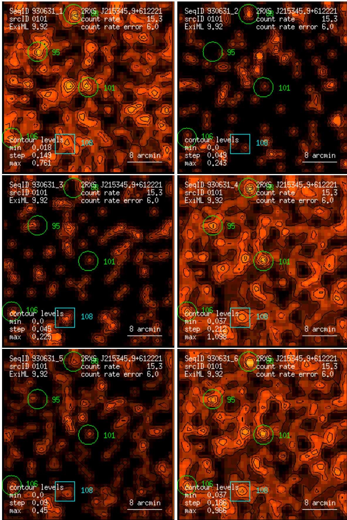
Figure 101: RASS 930631: detection 0101: band rate images, Gaussian filter: (1) PSPC channels 11 – 41, (2) 52 – 90, (3) 91 – 201, (4) 11 – 235, (5) 52 – 201, (6) 11 – 201. Broad band rates in counts/ks. Band rate contour levels in counts/ks/arcmin 2 .
