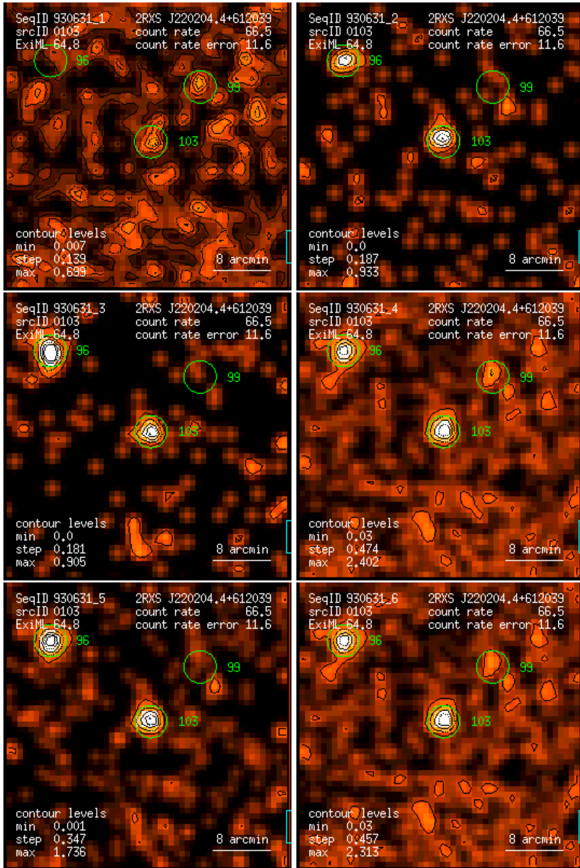
Figure 103: RASS 930631: detection 0103: band rate images, Gaussian filter: (1) PSPC channels 11 – 41, (2) 52 – 90, (3) 91 – 201, (4) 11 – 235, (5) 52 – 201, (6) 11 – 201. Broad band rates in counts/ks. Band rate contour levels in counts/ks/arcmin 2 .
