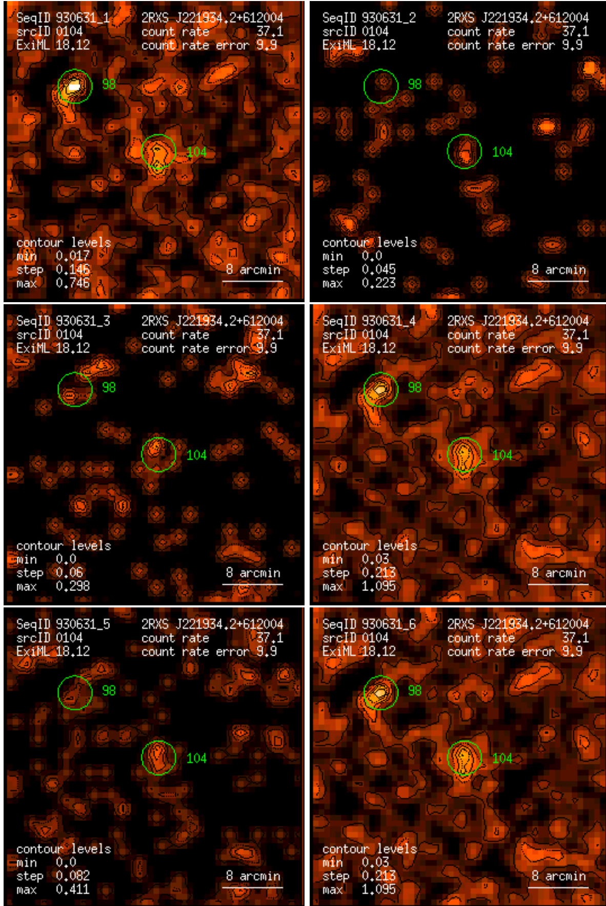
Figure 104: RASS 930631: detection 0104: band rate images, Gaussian filter: (1) PSPC channels 11 – 41, (2) 52 – 90, (3) 91 – 201, (4) 11 – 235, (5) 52 – 201, (6) 11 – 201. Broad band rates in counts/ks. Band rate contour levels in counts/ks/arcmin 2 .
