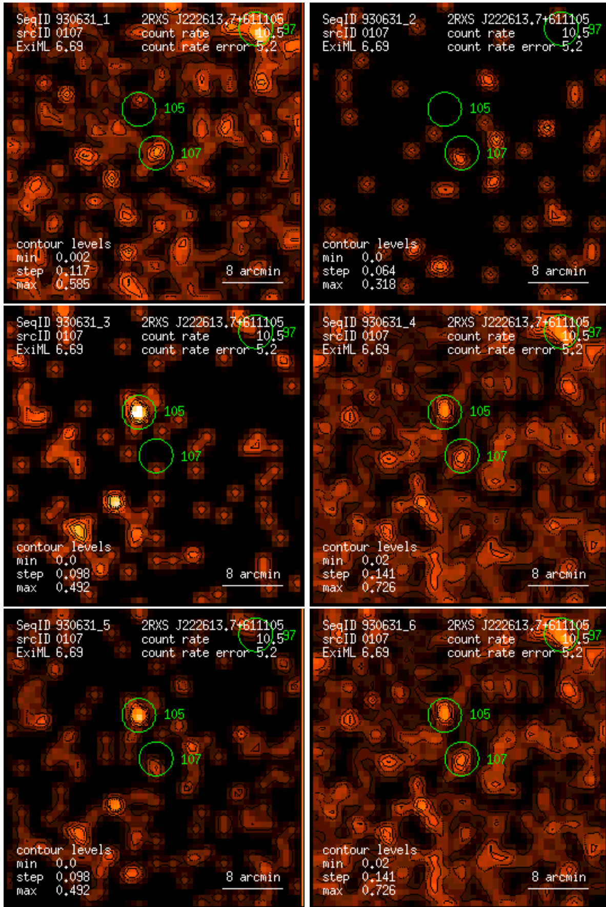
Figure 107: RASS 930631: detection 0107: band rate images, Gaussian filter: (1) PSPC channels 11 – 41, (2) 52 – 90, (3) 91 – 201, (4) 11 – 235, (5) 52 – 201, (6) 11 – 201. Broad band rates in counts/ks. Band rate contour levels in counts/ks/arcmin 2 .
