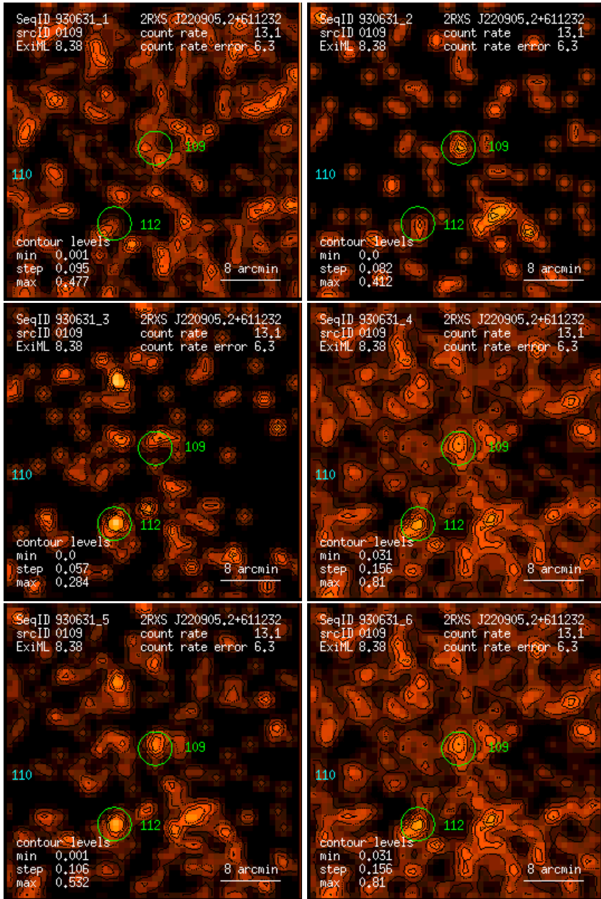
Figure 109: RASS 930631: detection 0109: band rate images, Gaussian filter: (1) PSPC channels 11 – 41, (2) 52 – 90, (3) 91 – 201, (4) 11 – 235, (5) 52 – 201, (6) 11 – 201. Broad band rates in counts/ks. Band rate contour levels in counts/ks/arcmin 2 .
