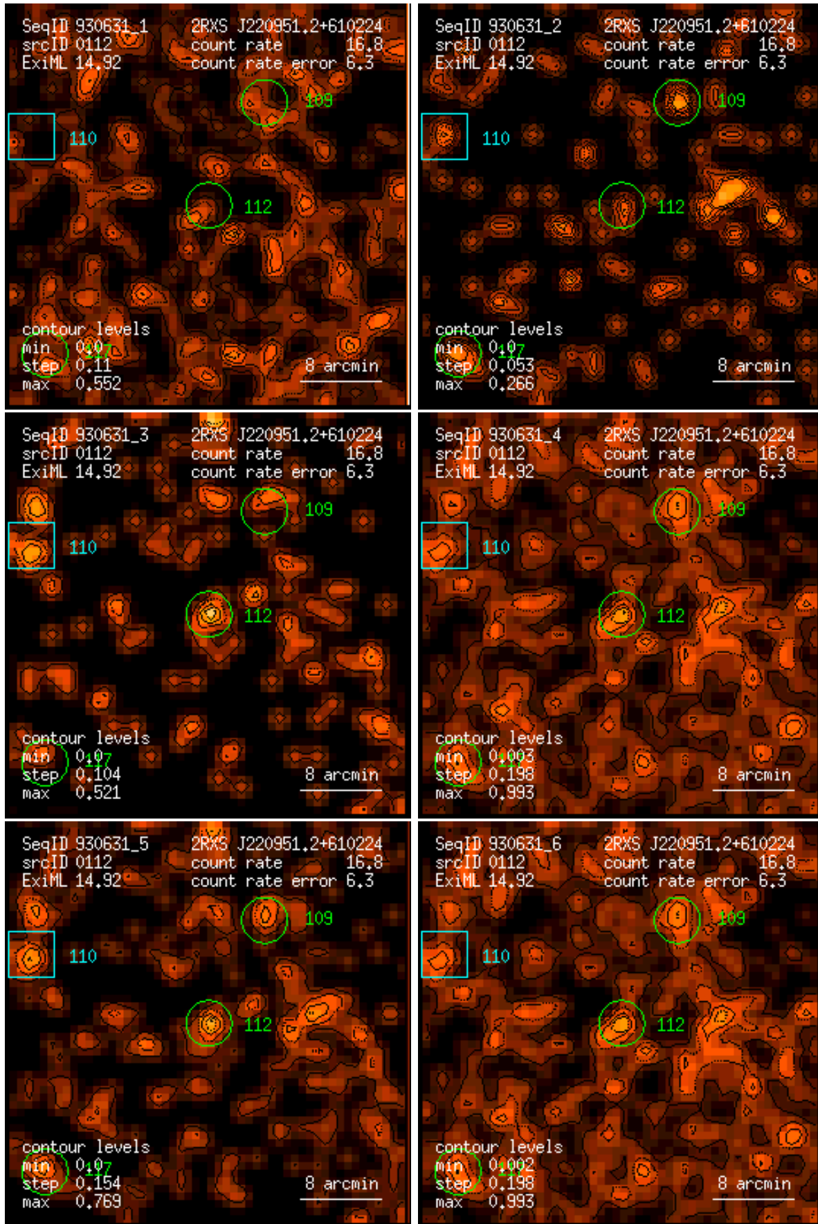
Figure 112: RASS 930631: detection 0112: band rate images, Gaussian filter: (1) PSPC channels 11 – 41, (2) 52 – 90, (3) 91 – 201, (4) 11 – 235, (5) 52 – 201, (6) 11 – 201. Broad band rates in counts/ks. Band rate contour levels in counts/ks/arcmin 2 .
