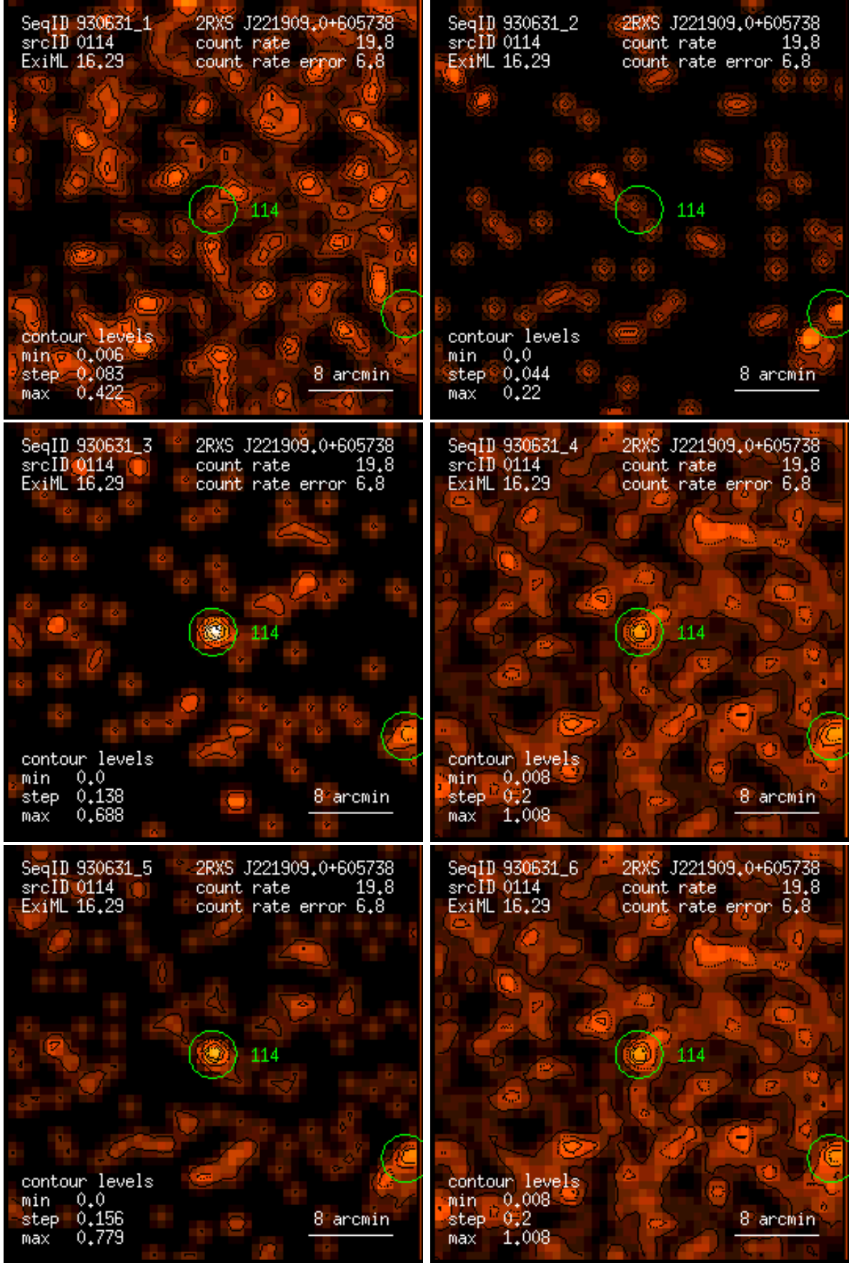
Figure 114: RASS 930631: detection 0114: band rate images, Gaussian filter: (1) PSPC channels 11 – 41, (2) 52 – 90, (3) 91 – 201, (4) 11 – 235, (5) 52 – 201, (6) 11 – 201. Broad band rates in counts/ks. Band rate contour levels in counts/ks/arcmin 2 .
