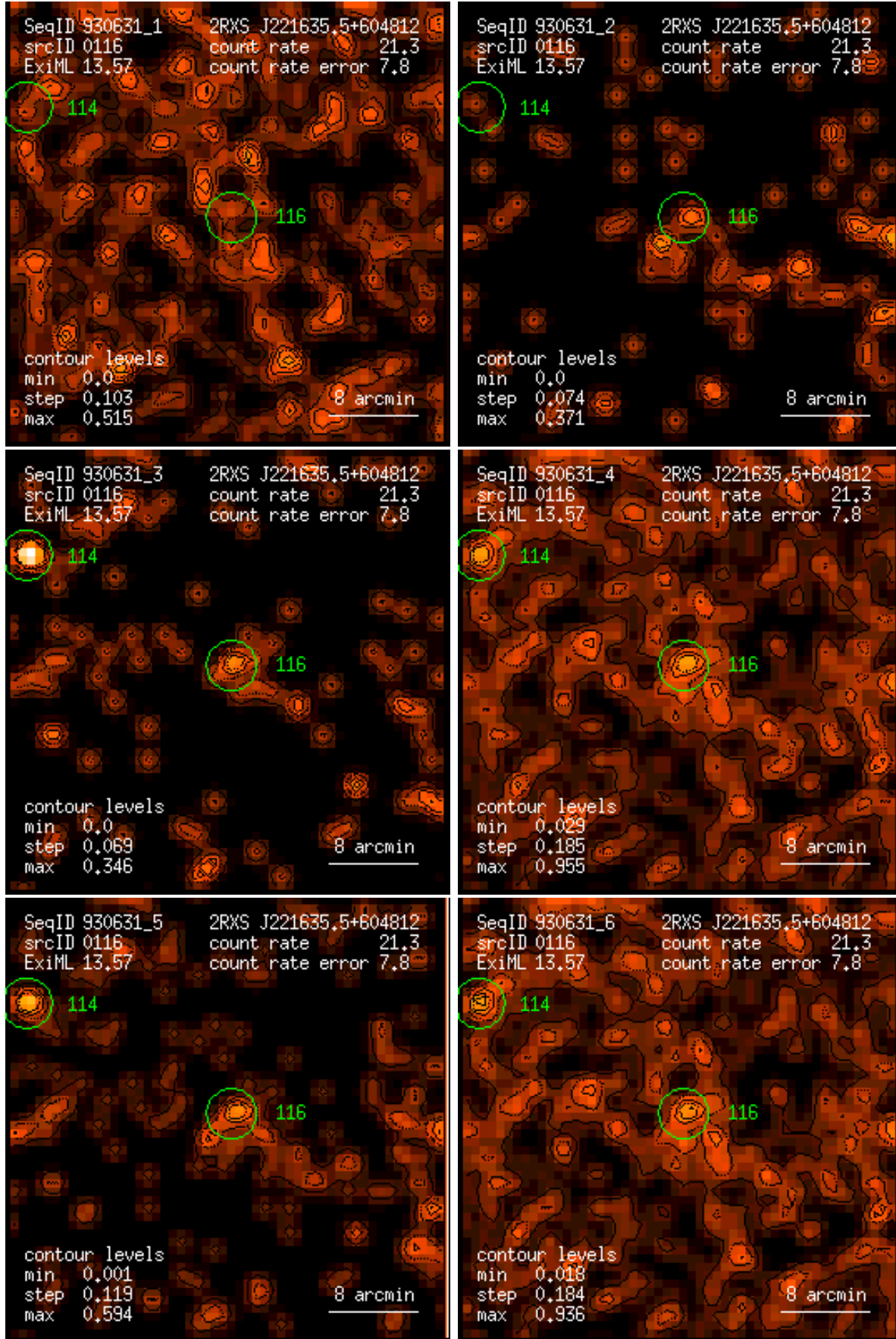
Figure 116: RASS 930631: detection 0116: band rate images, Gaussian filter: (1) PSPC channels 11 – 41, (2) 52 – 90, (3) 91 – 201, (4) 11 – 235, (5) 52 – 201, (6) 11 – 201. Broad band rates in counts/ks. Band rate contour levels in counts/ks/arcmin 2 .
