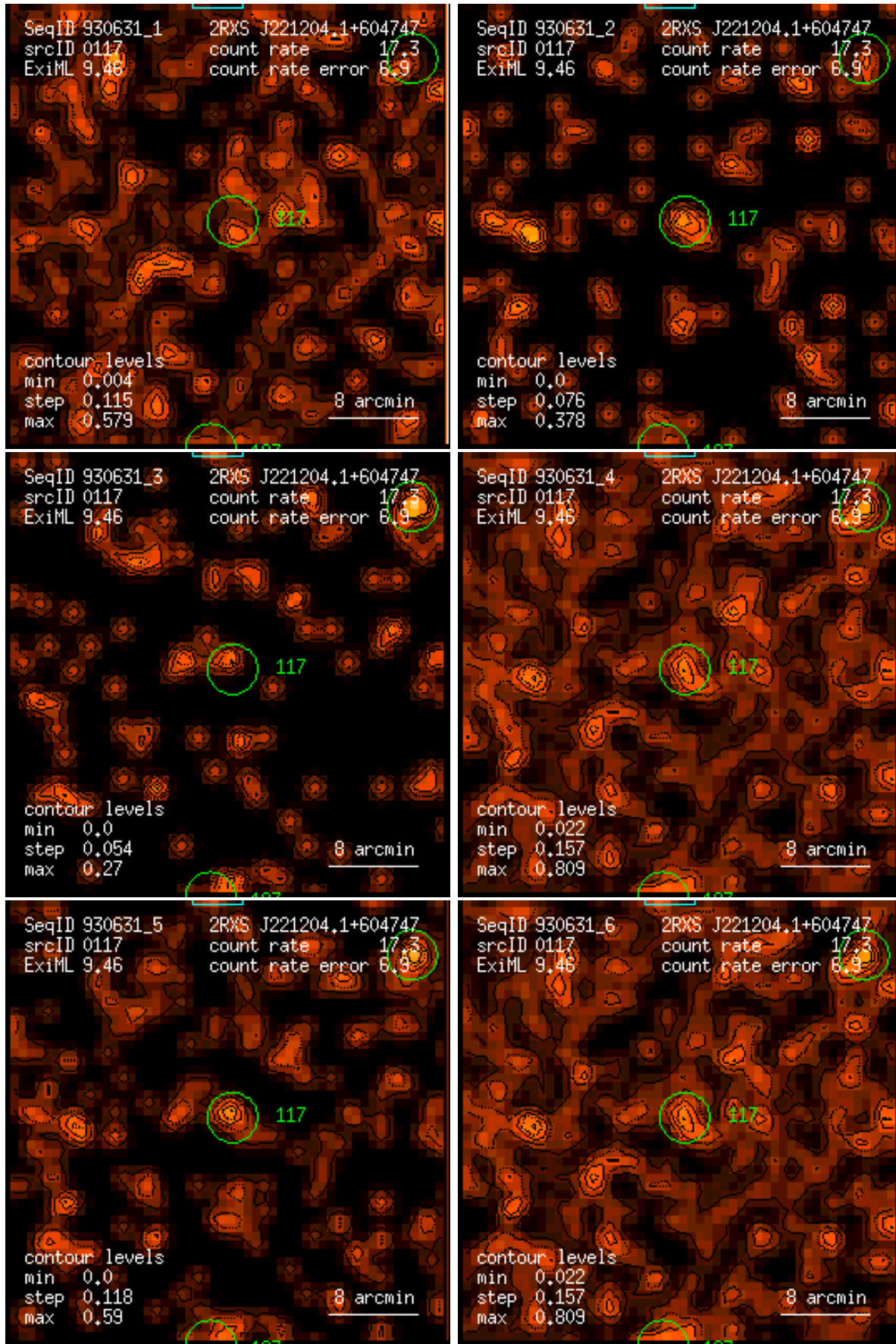
Figure 117: RASS 930631: detection 0117: band rate images, Gaussian filter: (1) PSPC channels 11 – 41, (2) 52 – 90, (3) 91 – 201, (4) 11 – 235, (5) 52 – 201, (6) 11 – 201. Broad band rates in counts/ks. Band rate contour levels in counts/ks/arcmin 2 .
