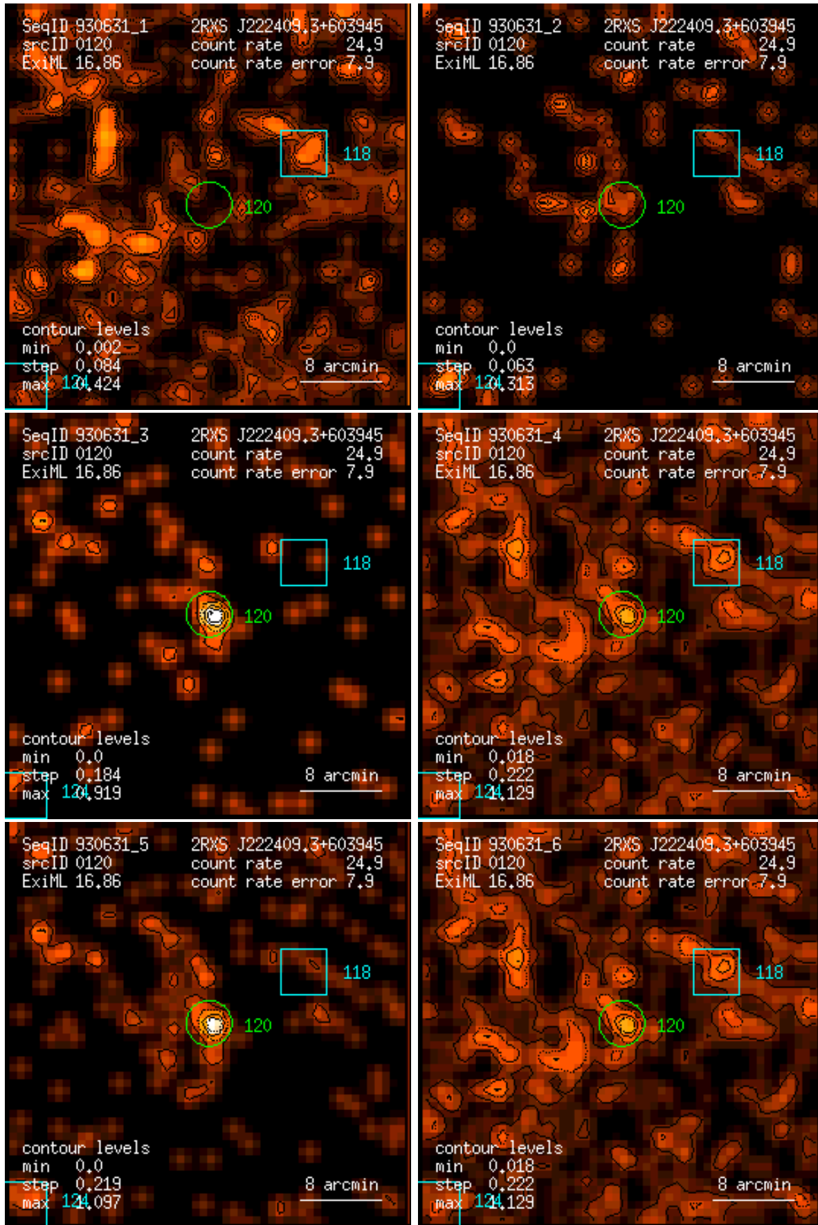
Figure 120: RASS 930631: detection 0120: band rate images, Gaussian filter: (1) PSPC channels 11 – 41, (2) 52 – 90, (3) 91 – 201, (4) 11 – 235, (5) 52 – 201, (6) 11 – 201. Broad band rates in counts/ks. Band rate contour levels in counts/ks/arcmin 2 .
