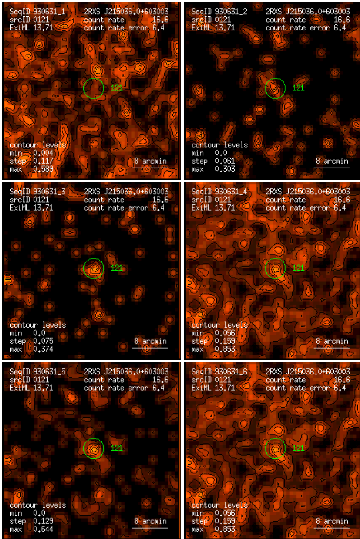
Figure 121: RASS 930631: detection 0121: band rate images, Gaussian filter: (1) PSPC channels 11 – 41, (2) 52 – 90, (3) 91 – 201, (4) 11 – 235, (5) 52 – 201, (6) 11 – 201. Broad band rates in counts/ks. Band rate contour levels in counts/ks/arcmin 2 .
