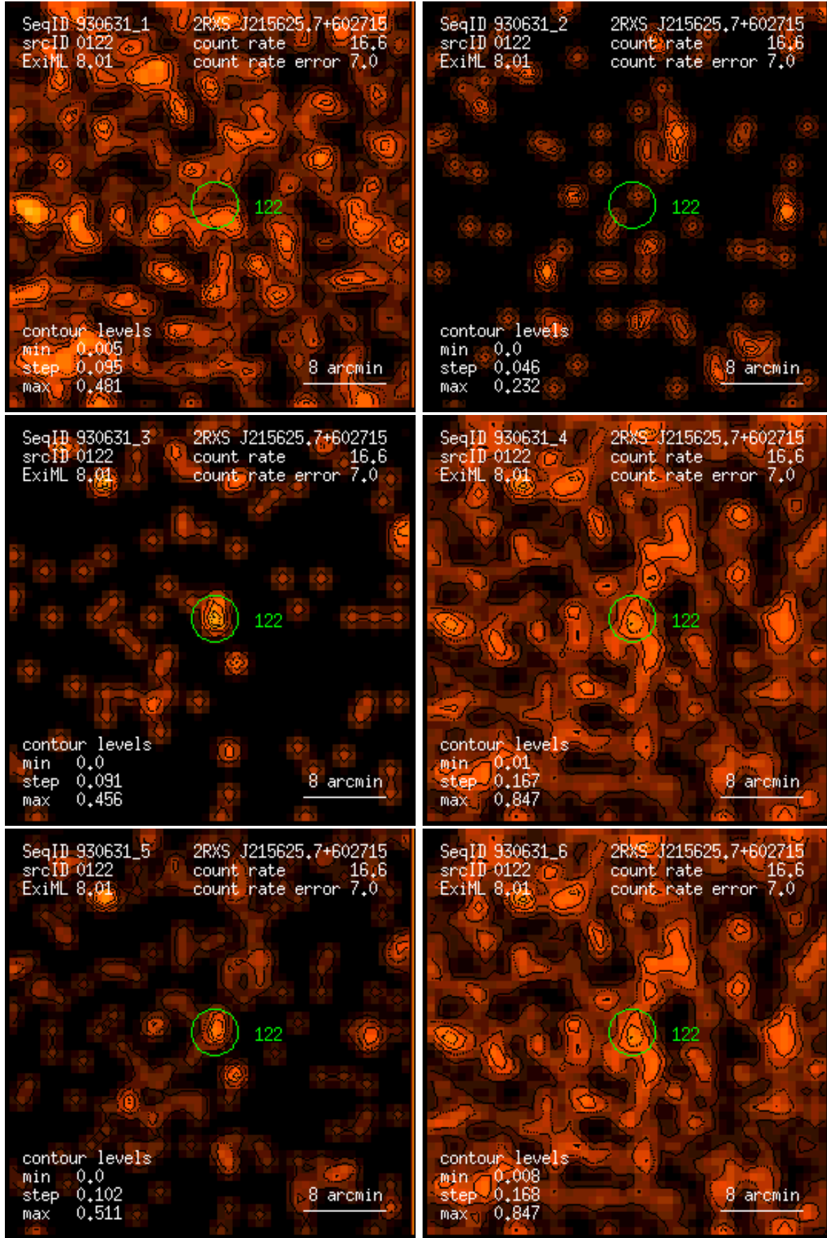
Figure 122: RASS 930631: detection 0122: band rate images, Gaussian filter: (1) PSPC channels 11 – 41, (2) 52 – 90, (3) 91 – 201, (4) 11 – 235, (5) 52 – 201, (6) 11 – 201. Broad band rates in counts/ks. Band rate contour levels in counts/ks/arcmin 2 .
