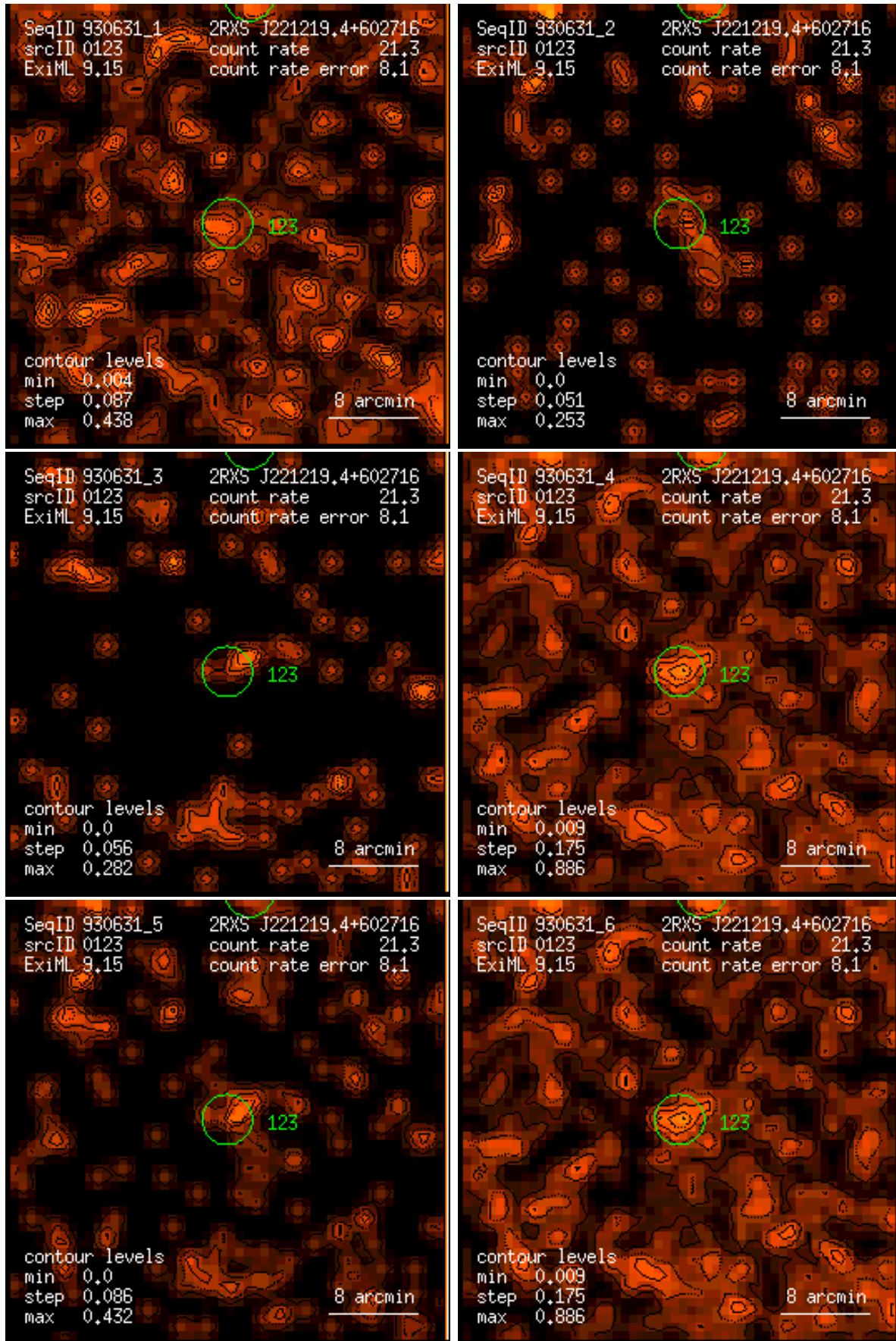
Figure 123: RASS 930631: detection 0123: band rate images, Gaussian filter: (1) PSPC channels 11 – 41, (2) 52 – 90, (3) 91 – 201, (4) 11 – 235, (5) 52 – 201, (6) 11 – 201. Broad band rates in counts/ks. Band rate contour levels in counts/ks/arcmin 2 .
