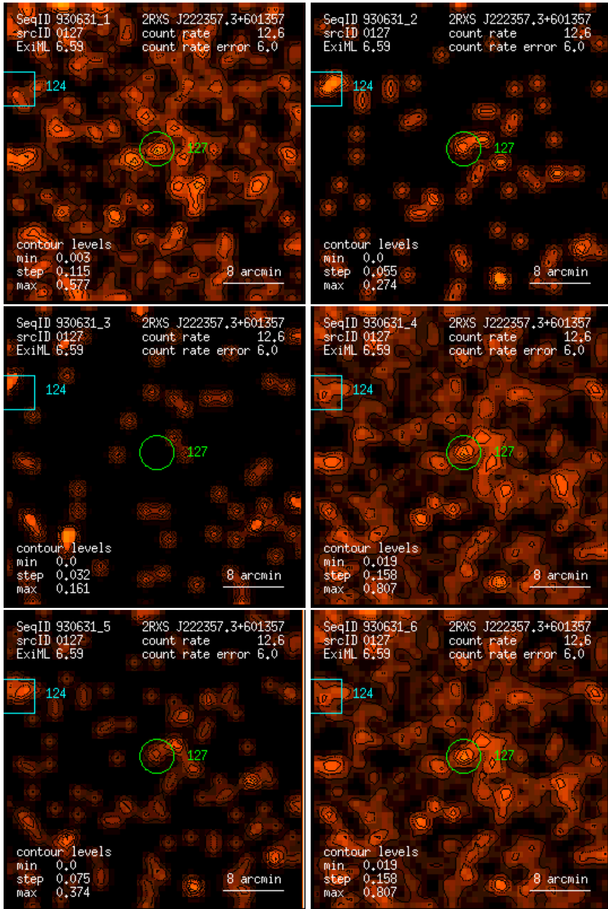
Figure 127: RASS 930631: detection 0127: band rate images, Gaussian filter: (1) PSPC channels 11 – 41, (2) 52 – 90, (3) 91 – 201, (4) 11 – 235, (5) 52 – 201, (6) 11 – 201. Broad band rates in counts/ks. Band rate contour levels in counts/ks/arcmin 2 .
