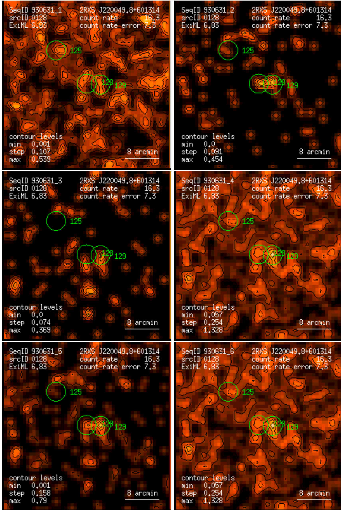
Figure 128: RASS 930631: detection 0128: band rate images, Gaussian filter: (1) PSPC channels 11 – 41, (2) 52 – 90, (3) 91 – 201, (4) 11 – 235, (5) 52 – 201, (6) 11 – 201. Broad band rates in counts/ks. Band rate contour levels in counts/ks/arcmin 2 .
