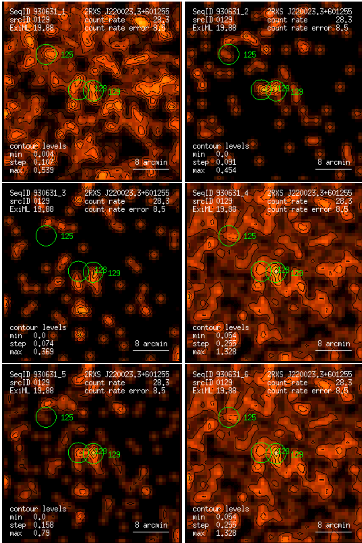
Figure 129: RASS 930631: detection 0129: band rate images, Gaussian filter: (1) PSPC channels 11 – 41, (2) 52 – 90, (3) 91 – 201, (4) 11 – 235, (5) 52 – 201, (6) 11 – 201. Broad band rates in counts/ks. Band rate contour levels in counts/ks/arcmin 2 .
