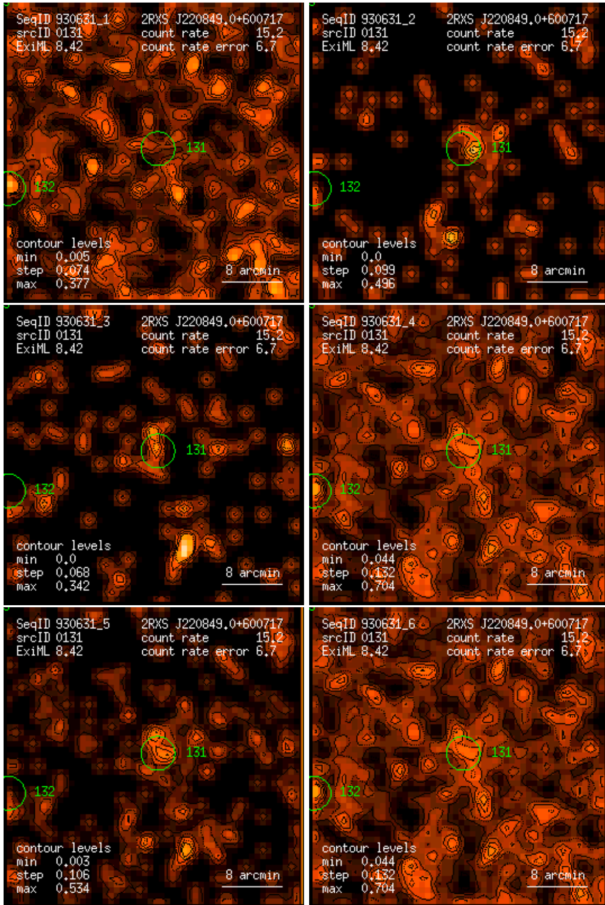
Figure 131: RASS 930631: detection 0131: band rate images, Gaussian filter: (1) PSPC channels 11 – 41, (2) 52 – 90, (3) 91 – 201, (4) 11 – 235, (5) 52 – 201, (6) 11 – 201. Broad band rates in counts/ks. Band rate contour levels in counts/ks/arcmin 2 .
