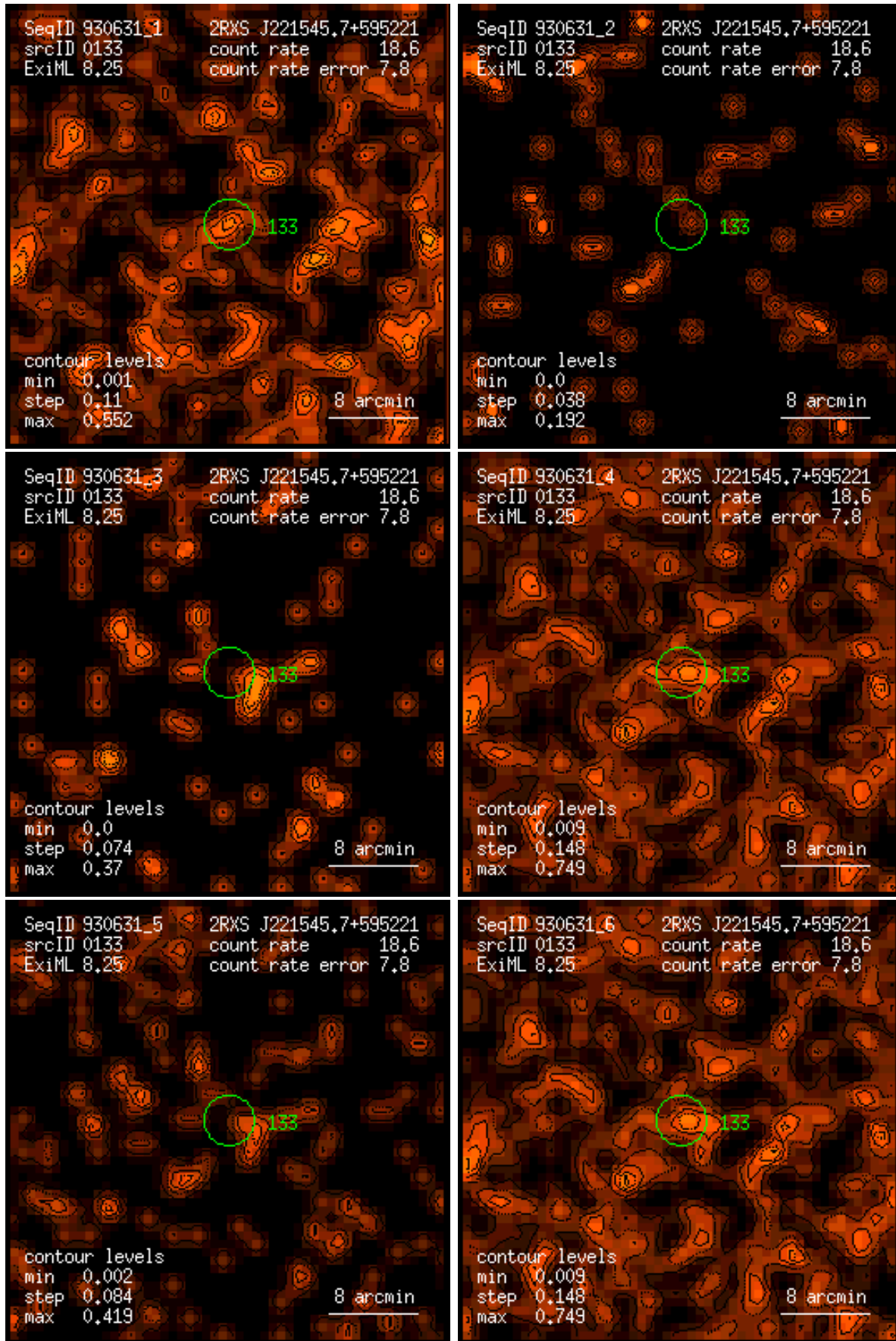
Figure 133: RASS 930631: detection 0133: band rate images, Gaussian filter: (1) PSPC channels 11 – 41, (2) 52 – 90, (3) 91 – 201, (4) 11 – 235, (5) 52 – 201, (6) 11 – 201. Broad band rates in counts/ks. Band rate contour levels in counts/ks/arcmin 2 .
