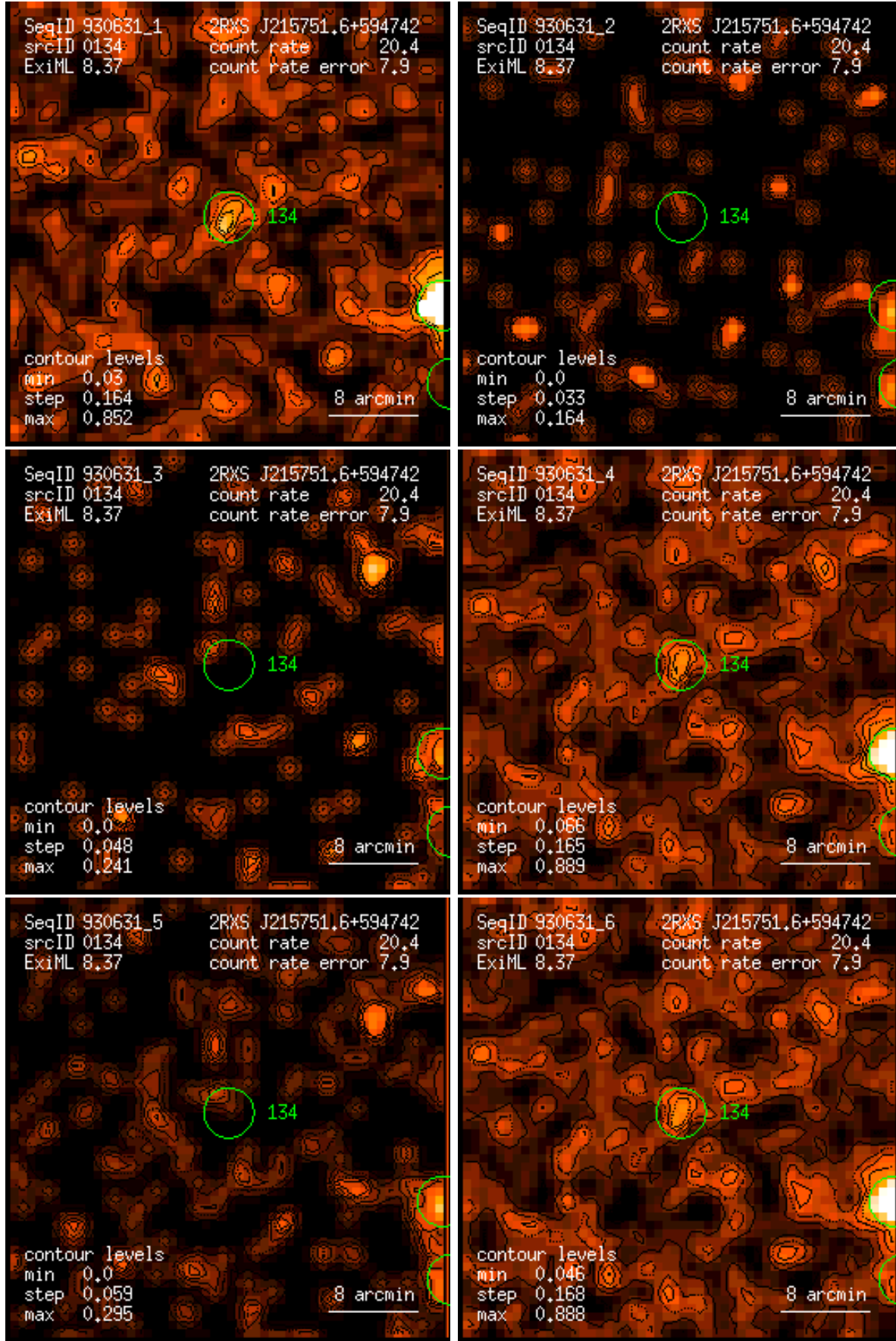
Figure 134: RASS 930631: detection 0134: band rate images, Gaussian filter: (1) PSPC channels 11 – 41, (2) 52 – 90, (3) 91 – 201, (4) 11 – 235, (5) 52 – 201, (6) 11 – 201. Broad band rates in counts/ks. Band rate contour levels in counts/ks/arcmin 2 .
