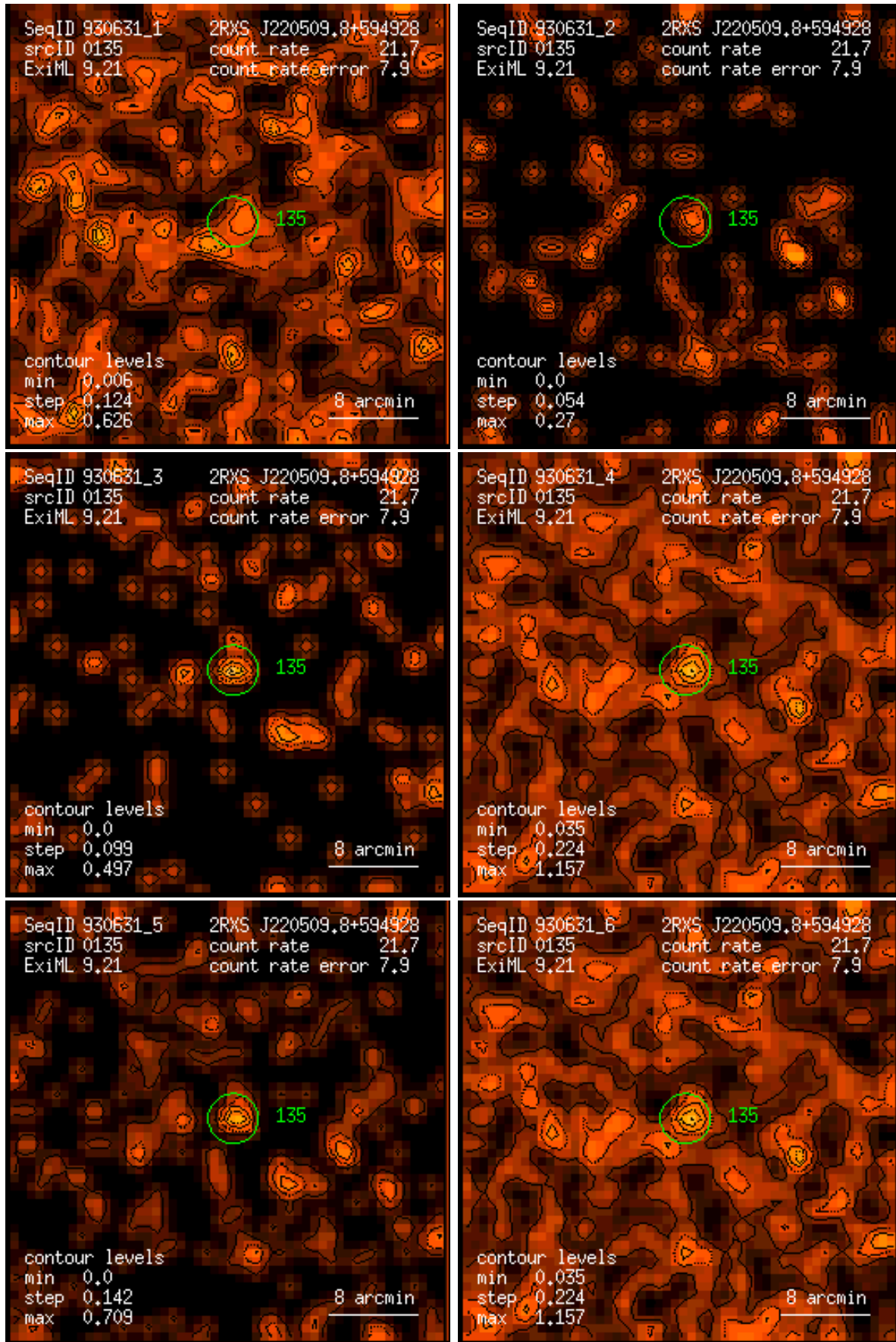
Figure 135: RASS 930631: detection 0135: band rate images, Gaussian filter: (1) PSPC channels 11 – 41, (2) 52 – 90, (3) 91 – 201, (4) 11 – 235, (5) 52 – 201, (6) 11 – 201. Broad band rates in counts/ks. Band rate contour levels in counts/ks/arcmin 2 .
