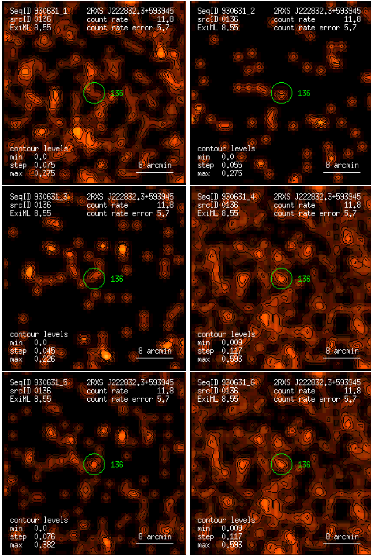
Figure 136: RASS 930631: detection 0136: band rate images, Gaussian filter: (1) PSPC channels 11 – 41, (2) 52 – 90, (3) 91 – 201, (4) 11 – 235, (5) 52 – 201, (6) 11 – 201. Broad band rates in counts/ks. Band rate contour levels in counts/ks/arcmin 2 .
