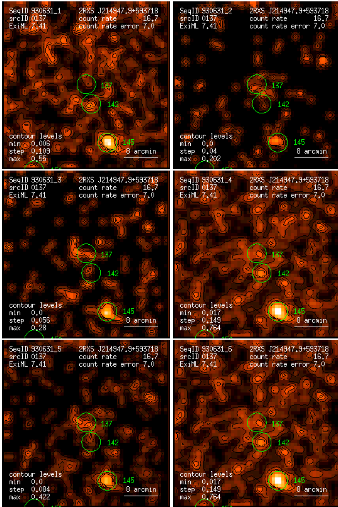
Figure 137: RASS 930631: detection 0137: band rate images, Gaussian filter: (1) PSPC channels 11 – 41, (2) 52 – 90, (3) 91 – 201, (4) 11 – 235, (5) 52 – 201, (6) 11 – 201. Broad band rates in counts/ks. Band rate contour levels in counts/ks/arcmin 2 .
