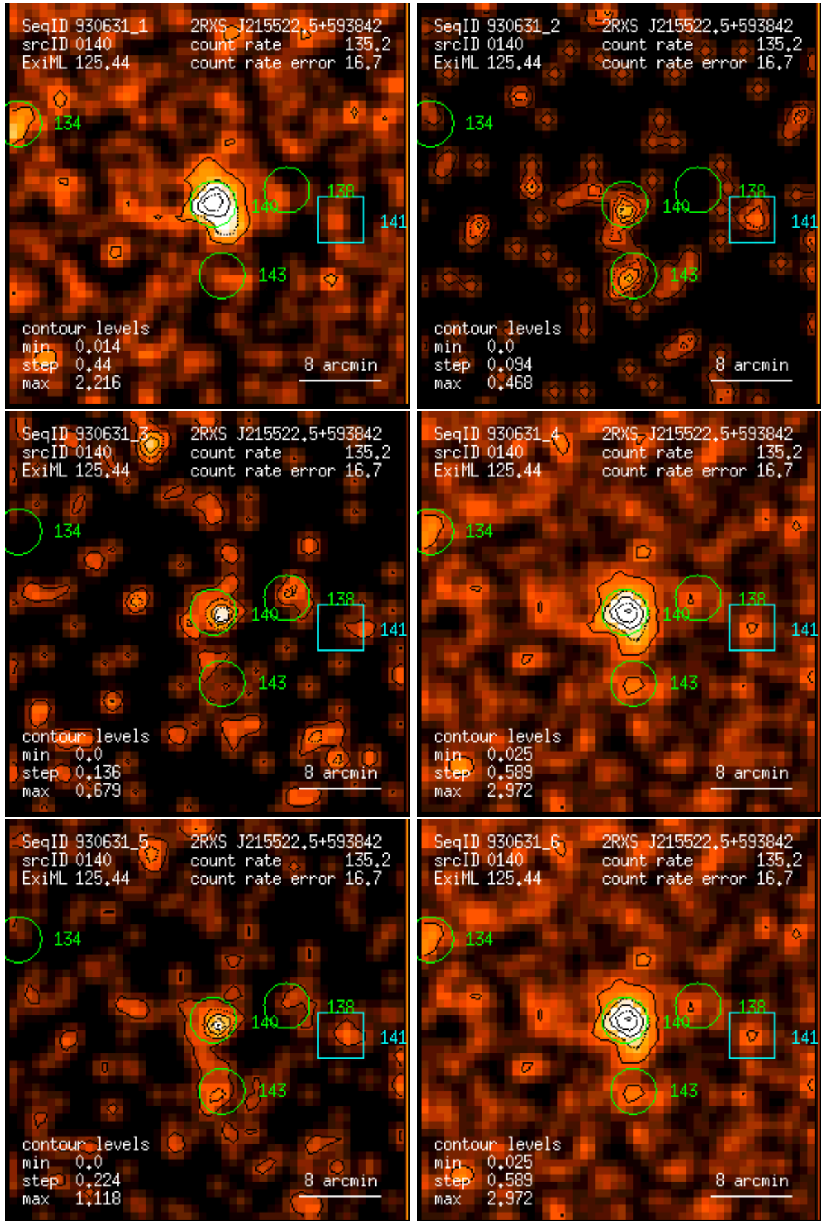
Figure 140: RASS 930631: detection 0140: band rate images, Gaussian filter: (1) PSPC channels 11 – 41, (2) 52 – 90, (3) 91 – 201, (4) 11 – 235, (5) 52 – 201, (6) 11 – 201. Broad band rates in counts/ks. Band rate contour levels in counts/ks/arcmin 2 .
