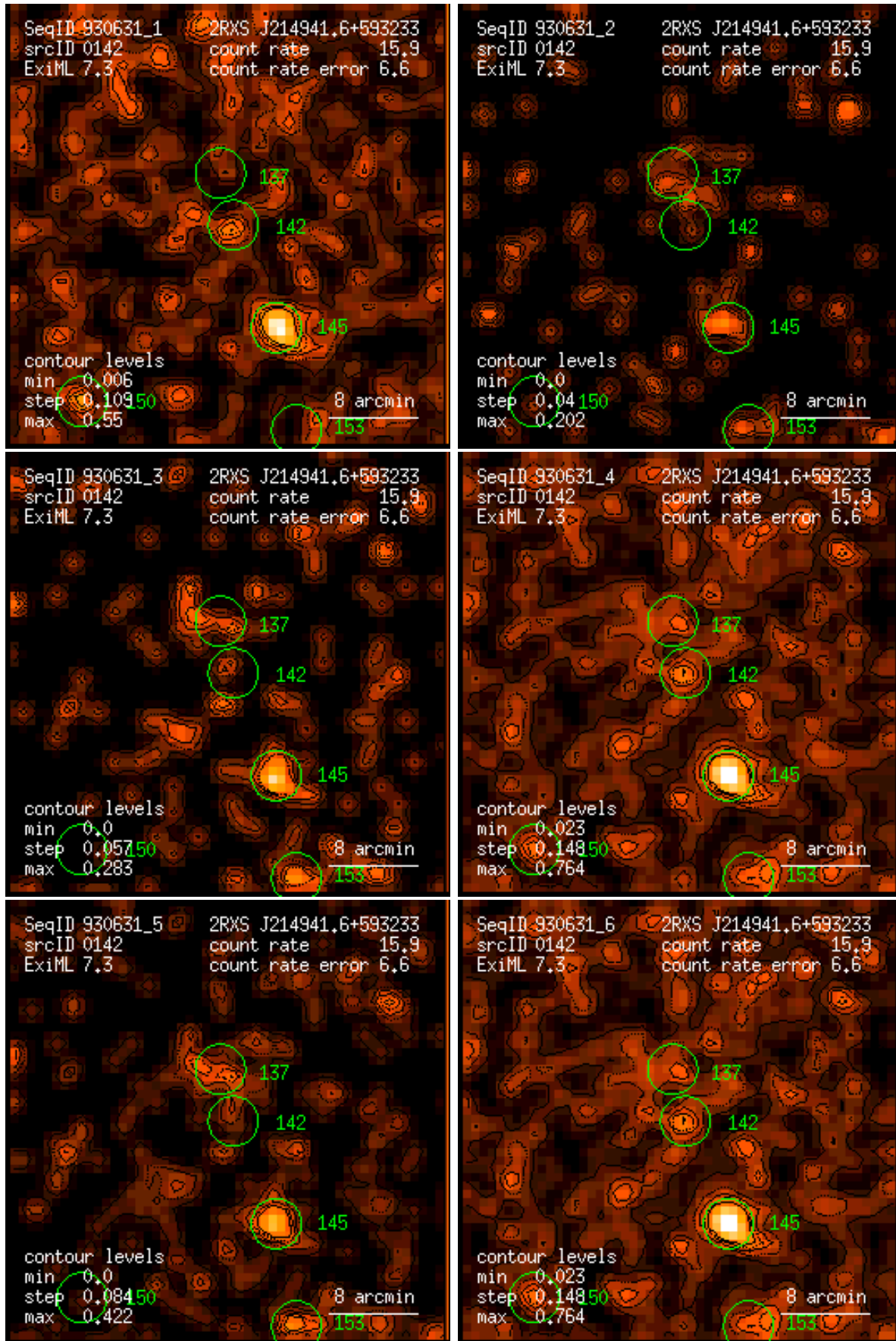
Figure 142: RASS 930631: detection 0142: band rate images, Gaussian filter: (1) PSPC channels 11 – 41, (2) 52 – 90, (3) 91 – 201, (4) 11 – 235, (5) 52 – 201, (6) 11 – 201. Broad band rates in counts/ks. Band rate contour levels in counts/ks/arcmin 2 .
