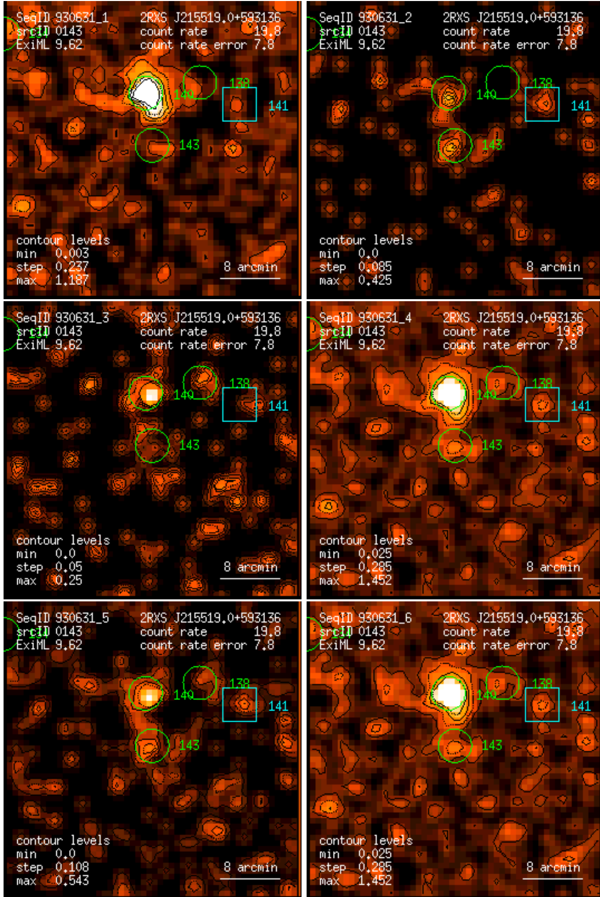
Figure 143: RASS 930631: detection 0143: band rate images, Gaussian filter: (1) PSPC channels 11 – 41, (2) 52 – 90, (3) 91 – 201, (4) 11 – 235, (5) 52 – 201, (6) 11 – 201. Broad band rates in counts/ks. Band rate contour levels in counts/ks/arcmin 2 .
