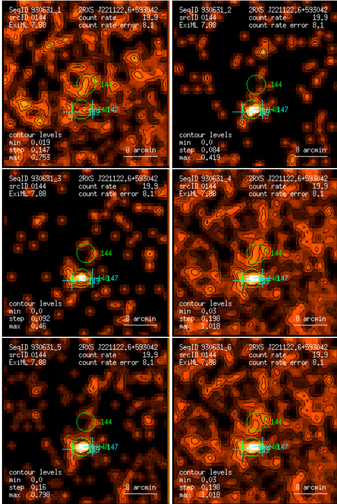
Figure 144: RASS 930631: detection 0144: band rate images, Gaussian filter: (1) PSPC channels 11 – 41, (2) 52 – 90, (3) 91 – 201, (4) 11 – 235, (5) 52 – 201, (6) 11 – 201. Broad band rates in counts/ks. Band rate contour levels in counts/ks/arcmin 2 .
