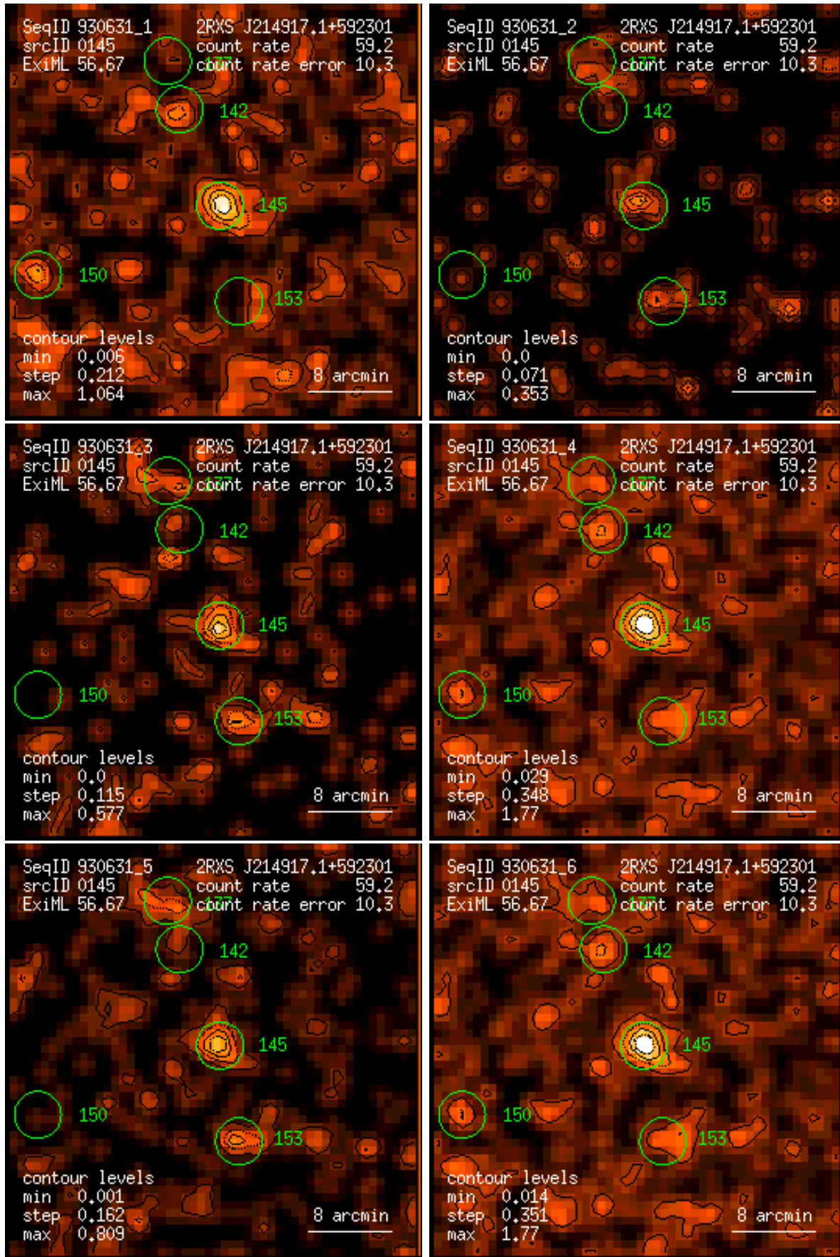
Figure 145: RASS 930631: detection 0145: band rate images, Gaussian filter: (1) PSPC channels 11 – 41, (2) 52 – 90, (3) 91 – 201, (4) 11 – 235, (5) 52 – 201, (6) 11 – 201. Broad band rates in counts/ks. Band rate contour levels in counts/ks/arcmin 2 .
