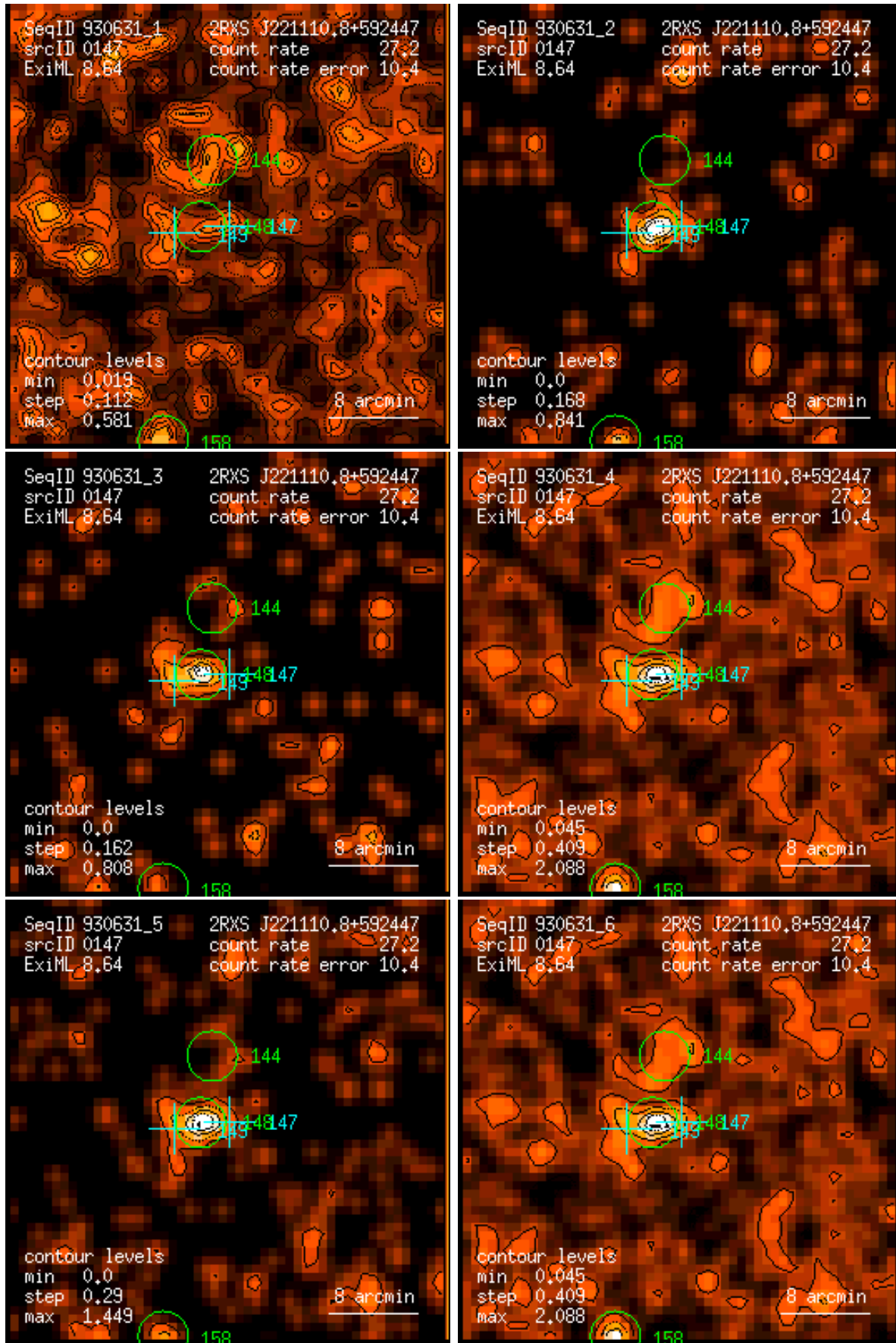
Figure 147: RASS 930631: detection 0147: band rate images, Gaussian filter: (1) PSPC channels 11 – 41, (2) 52 – 90, (3) 91 – 201, (4) 11 – 235, (5) 52 – 201, (6) 11 – 201. Broad band rates in counts/ks. Band rate contour levels in counts/ks/arcmin 2 .
