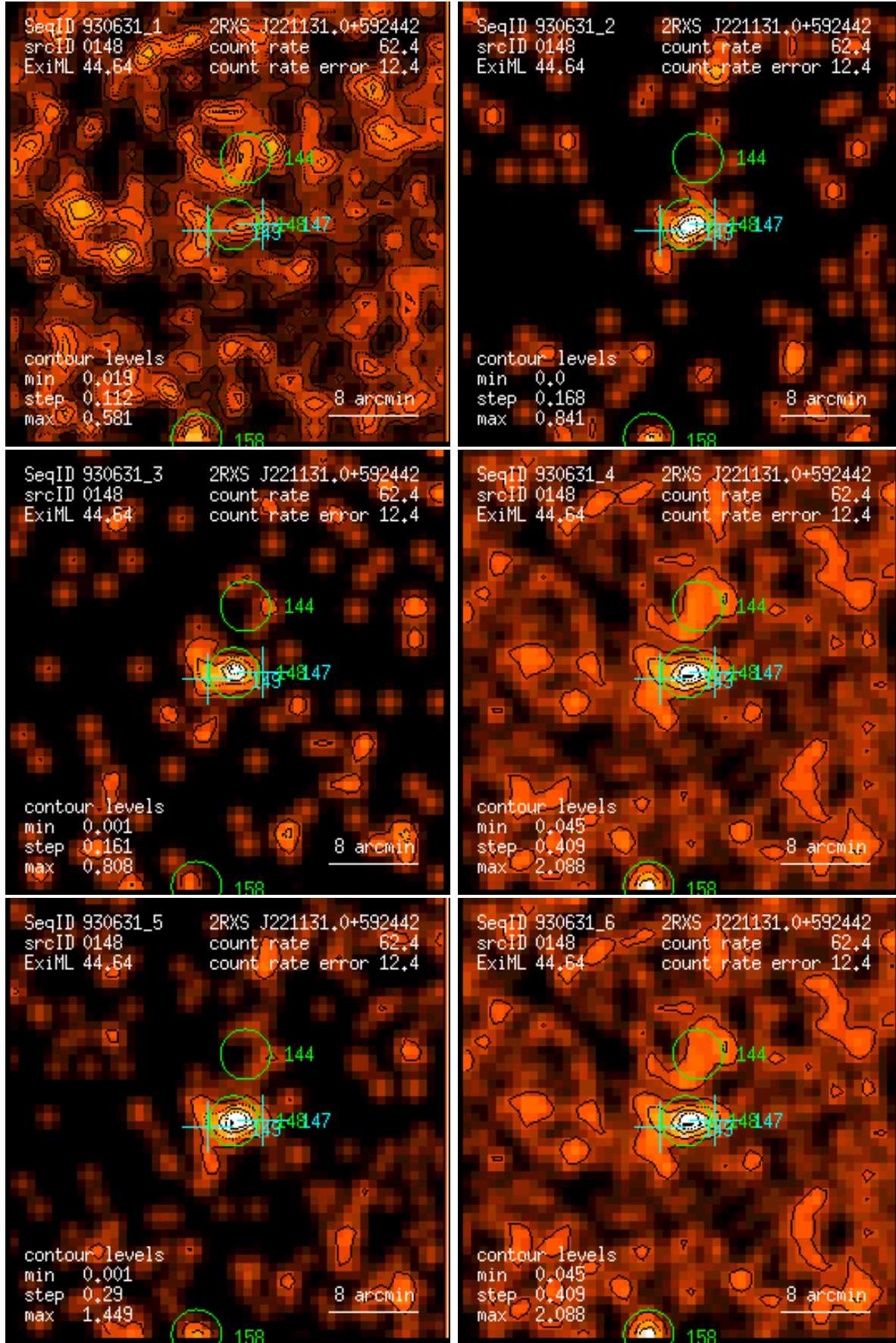
Figure 148: RASS 930631: detection 0148: band rate images, Gaussian filter: (1) PSPC channels 11 – 41, (2) 52 – 90, (3) 91 – 201, (4) 11 – 235, (5) 52 – 201, (6) 11 – 201. Broad band rates in counts/ks. Band rate contour levels in counts/ks/arcmin 2 .
