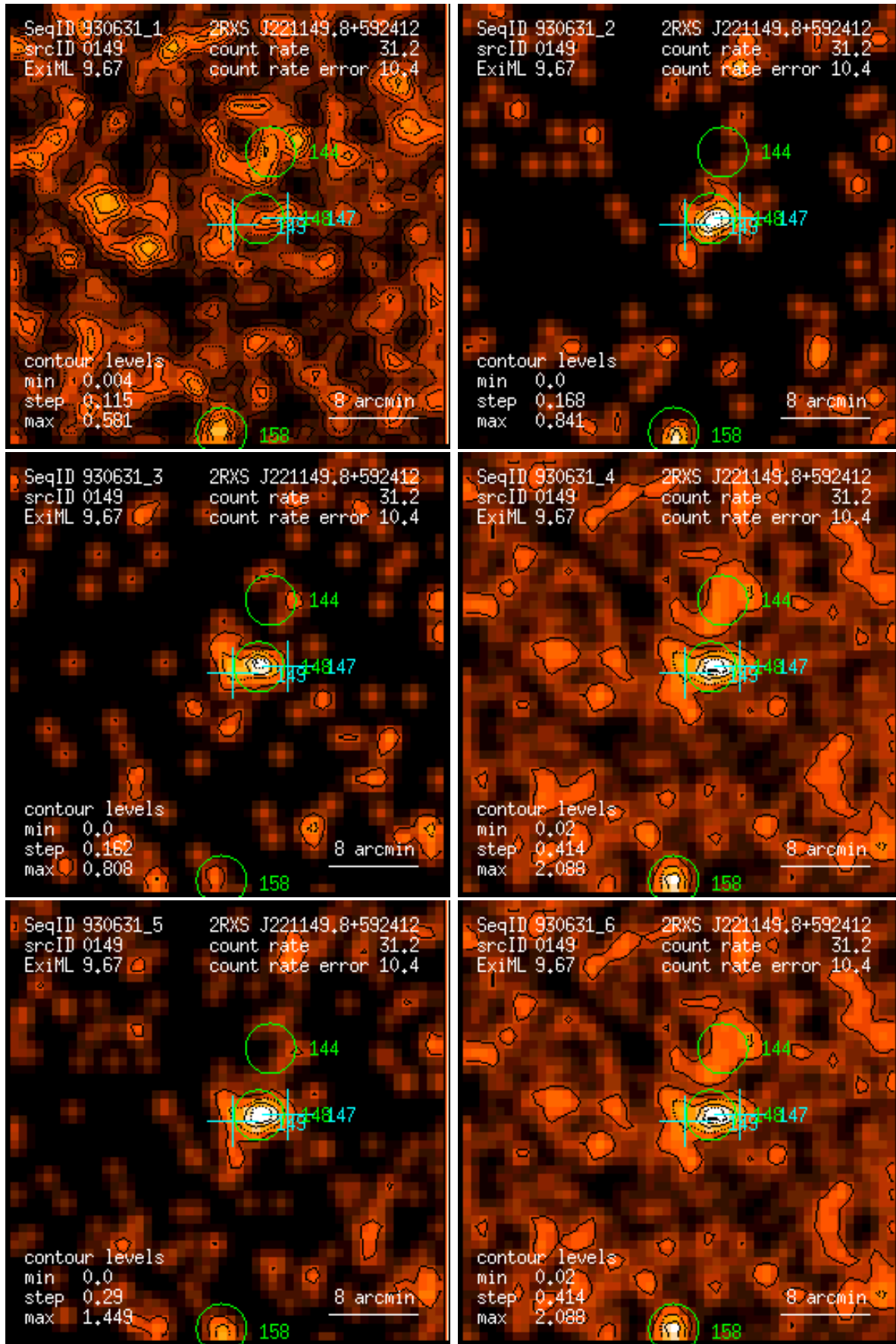
Figure 149: RASS 930631: detection 0149: band rate images, Gaussian filter: (1) PSPC channels 11 – 41, (2) 52 – 90, (3) 91 – 201, (4) 11 – 235, (5) 52 – 201, (6) 11 – 201. Broad band rates in counts/ks. Band rate contour levels in counts/ks/arcmin 2 .
