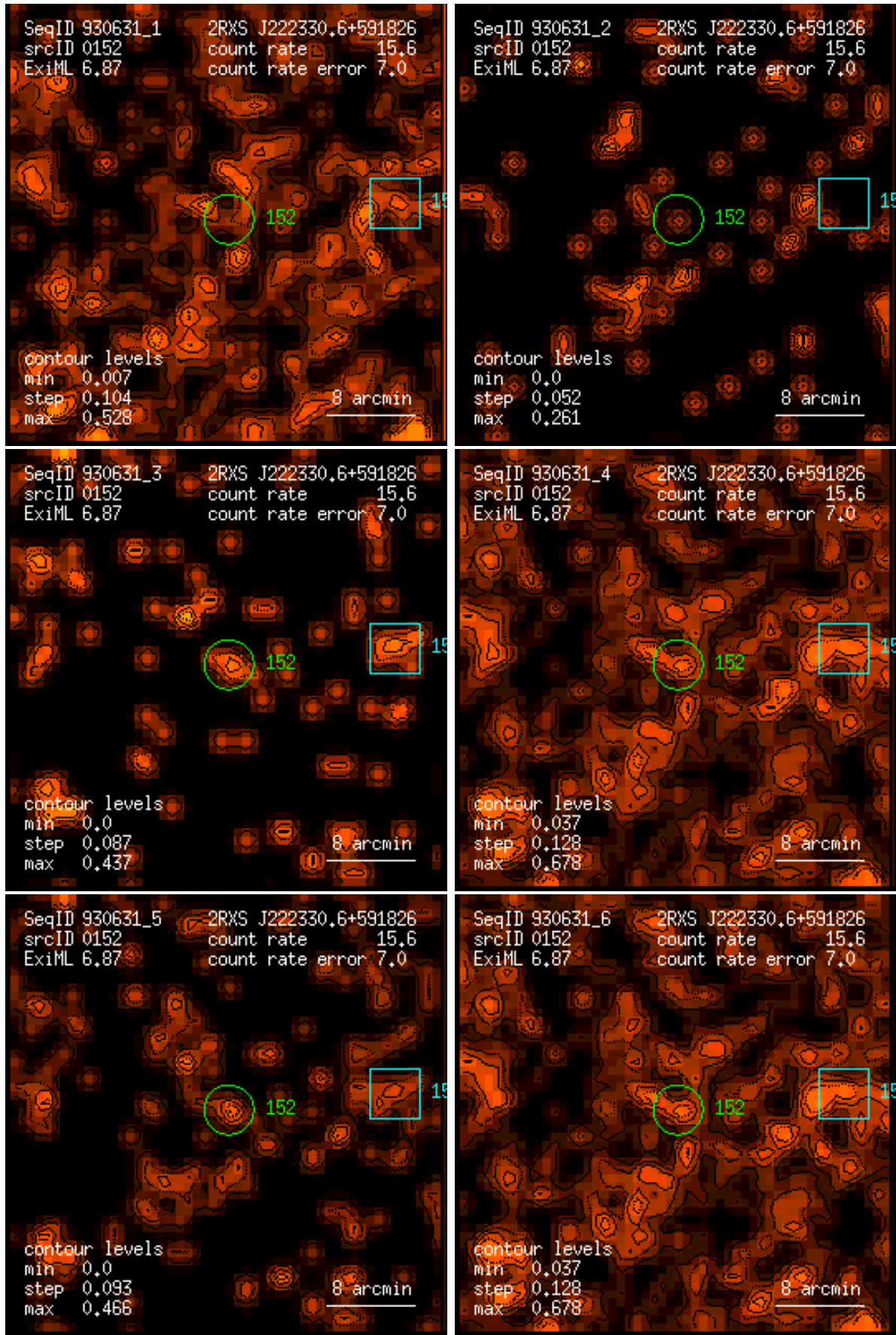
Figure 152: RASS 930631: detection 0152: band rate images, Gaussian filter: (1) PSPC channels 11 – 41, (2) 52 – 90, (3) 91 – 201, (4) 11 – 235, (5) 52 – 201, (6) 11 – 201. Broad band rates in counts/ks. Band rate contour levels in counts/ks/arcmin 2 .
