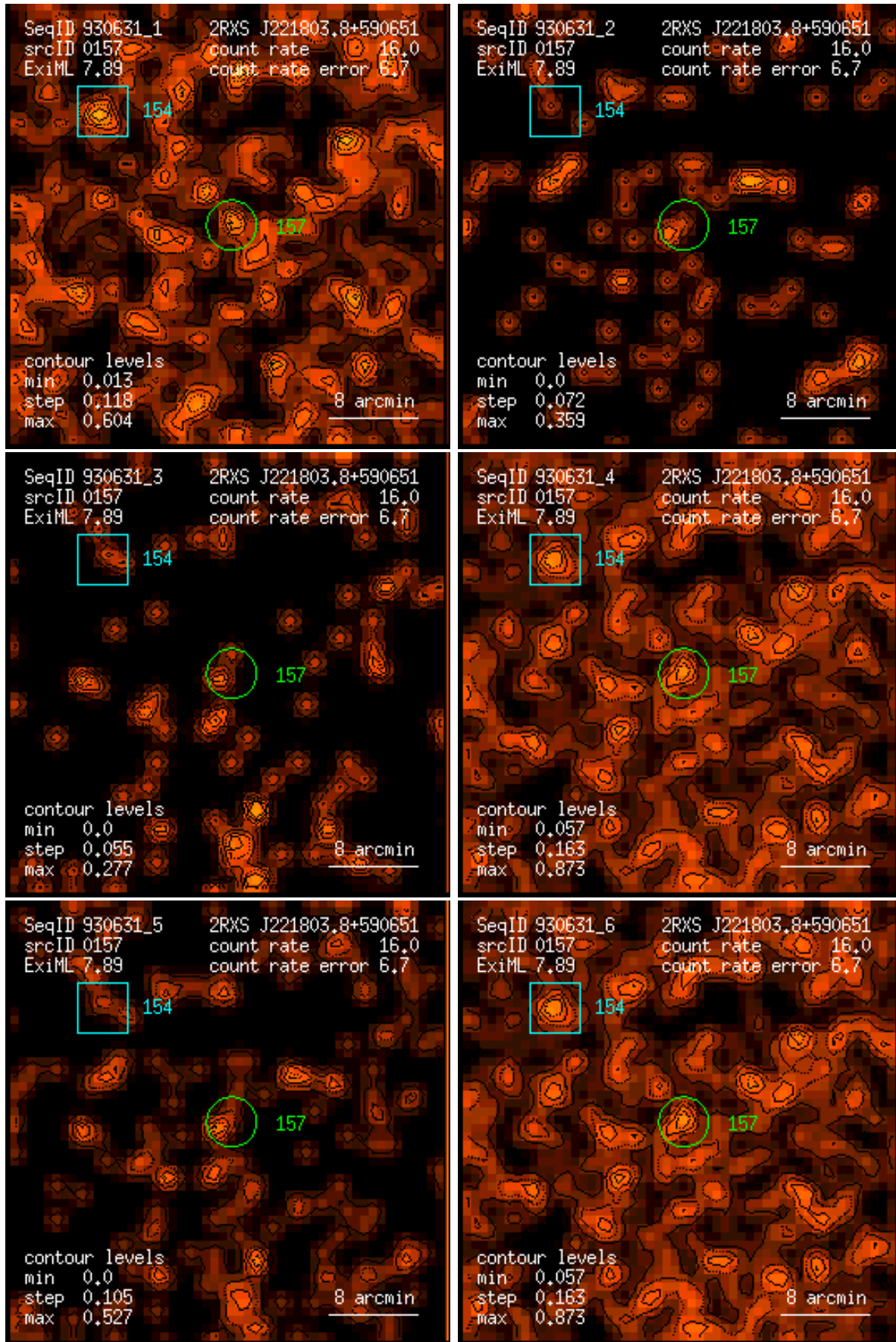
Figure 157: RASS 930631: detection 0157: band rate images, Gaussian filter: (1) PSPC channels 11 – 41, (2) 52 – 90, (3) 91 – 201, (4) 11 – 235, (5) 52 – 201, (6) 11 – 201. Broad band rates in counts/ks. Band rate contour levels in counts/ks/arcmin 2 .
