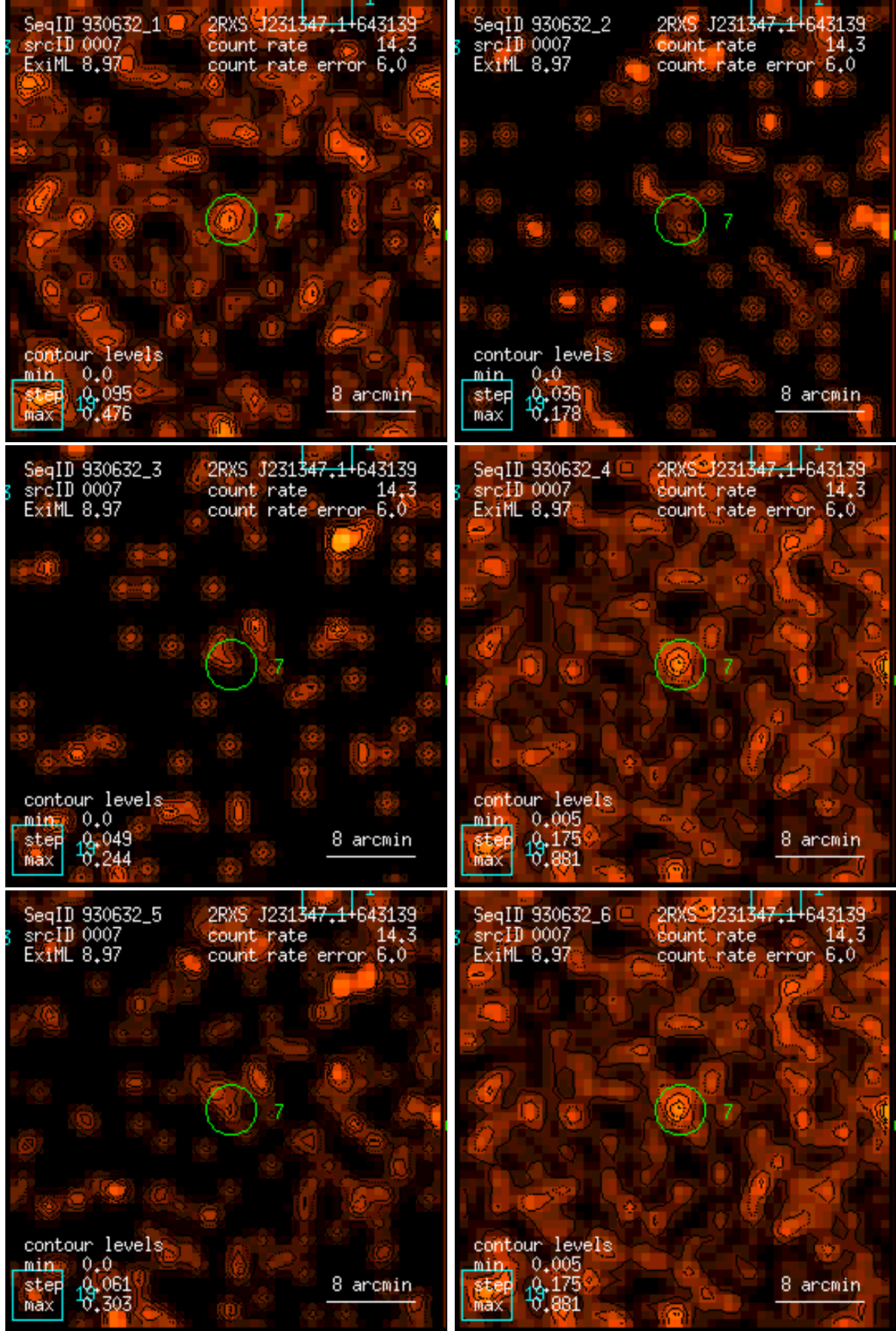
Figure 7: RASS 930632: detection 0007: band rate images, Gaussian filter: (1) PSPC channels 11 – 41, (2) 52 – 90, (3) 91 – 201, (4) 11 – 235, (5) 52 – 201, (6) 11 – 201. Broad band rates in counts/ks. Band rate contour levels in counts/ks/arcmin 2 .
