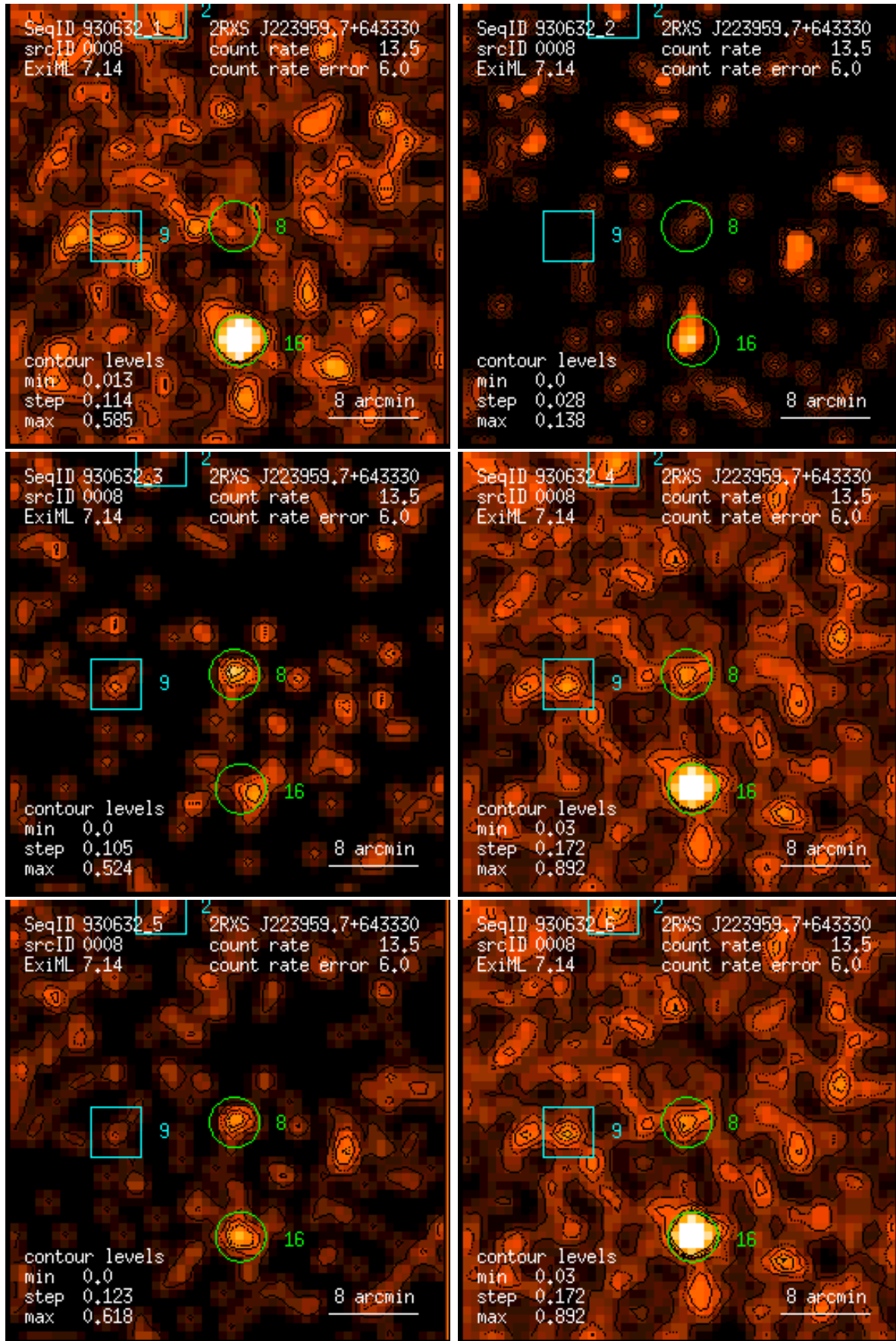
Figure 8: RASS 930632: detection 0008: band rate images, Gaussian filter: (1) PSPC channels 11 – 41, (2) 52 – 90, (3) 91 – 201, (4) 11 – 235, (5) 52 – 201, (6) 11 – 201. Broad band rates in counts/ks. Band rate contour levels in counts/ks/arcmin 2 .
