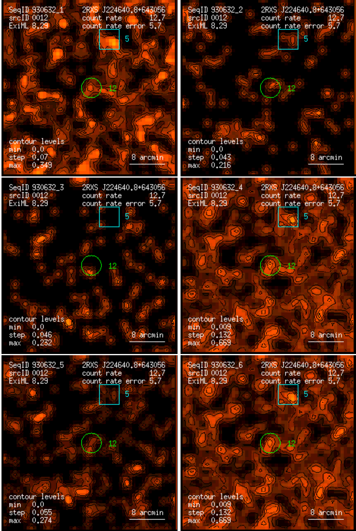
Figure 12: RASS 930632: detection 0012: band rate images, Gaussian filter: (1) PSPC channels 11 – 41, (2) 52 – 90, (3) 91 – 201, (4) 11 – 235, (5) 52 – 201, (6) 11 – 201. Broad band rates in counts/ks. Band rate contour levels in counts/ks/arcmin 2 .
