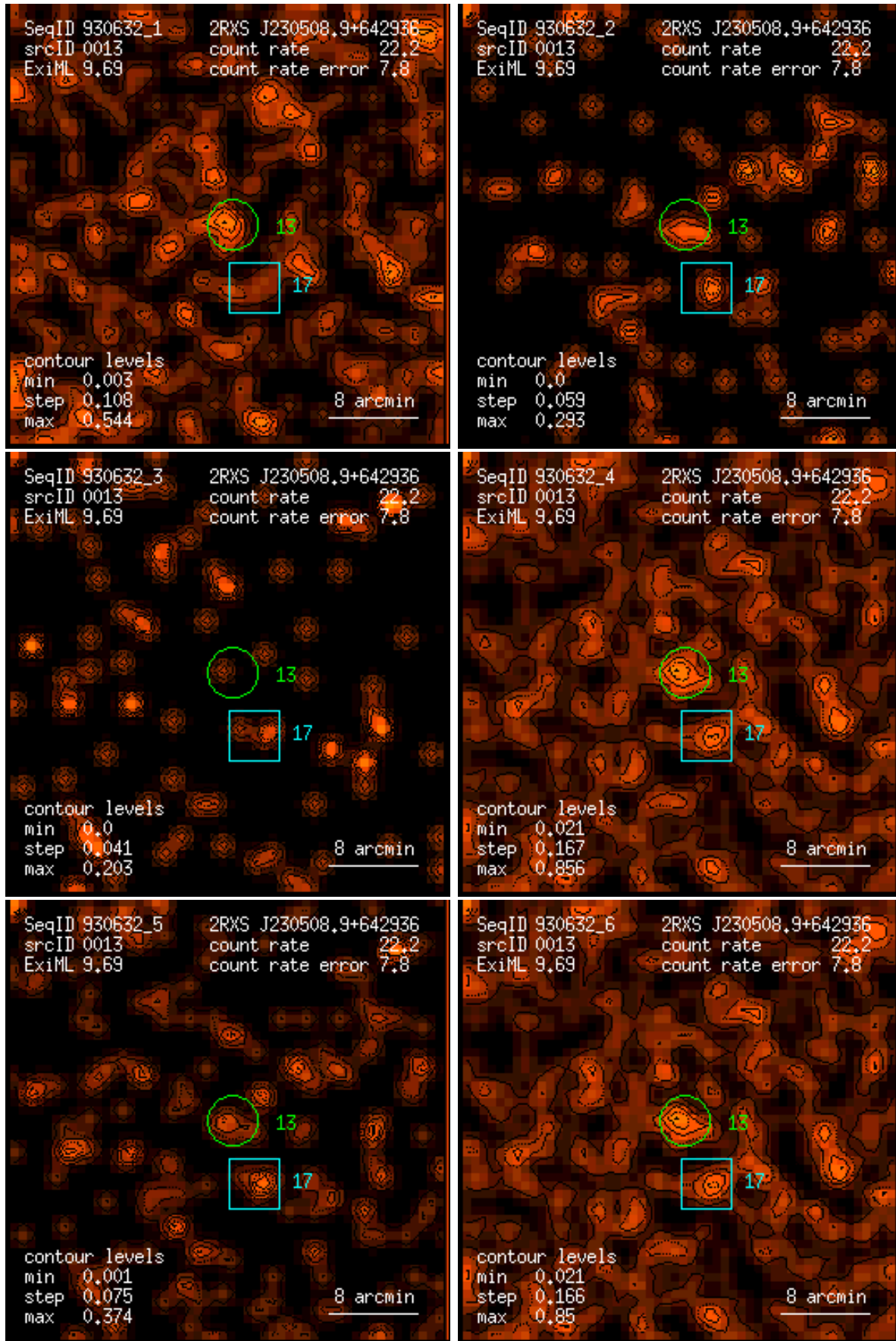
Figure 13: RASS 930632: detection 0013: band rate images, Gaussian filter: (1) PSPP channels 11 – 41, (2) 52 – 90, (3) 91 – 201, (4) 11 – 235, (5) 52 – 201, (6) 11 – 201. Broad band rates in counts/ks. Band rate contour levels in counts/ks/arcmin 2 .
