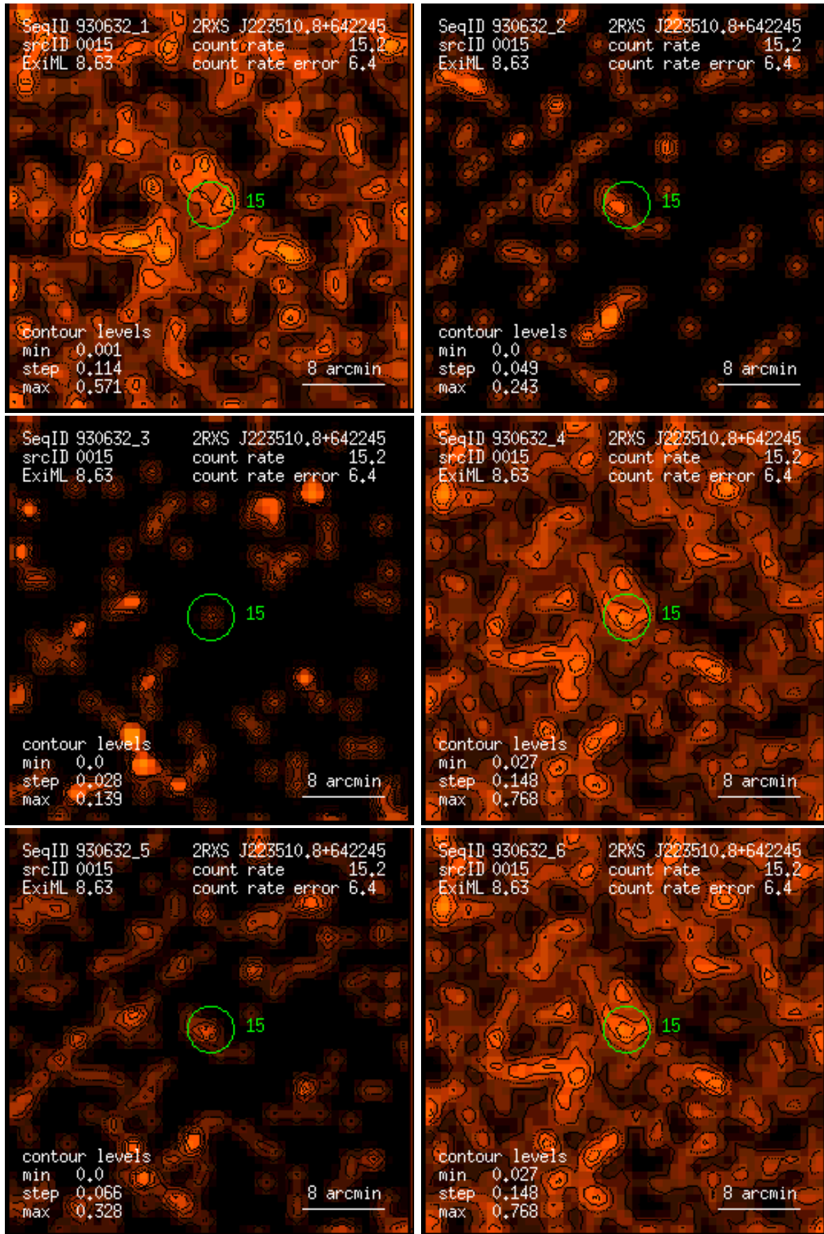
Figure 15: RASS 930632: detection 0015: band rate images, Gaussian filter: (1) PSPC channels 11 – 41, (2) 52 – 90, (3) 91 – 201, (4) 11 – 235, (5) 52 – 201, (6) 11 – 201. Broad band rates in counts/ks. Band rate contour levels in counts/ks/arcmin 2 .
