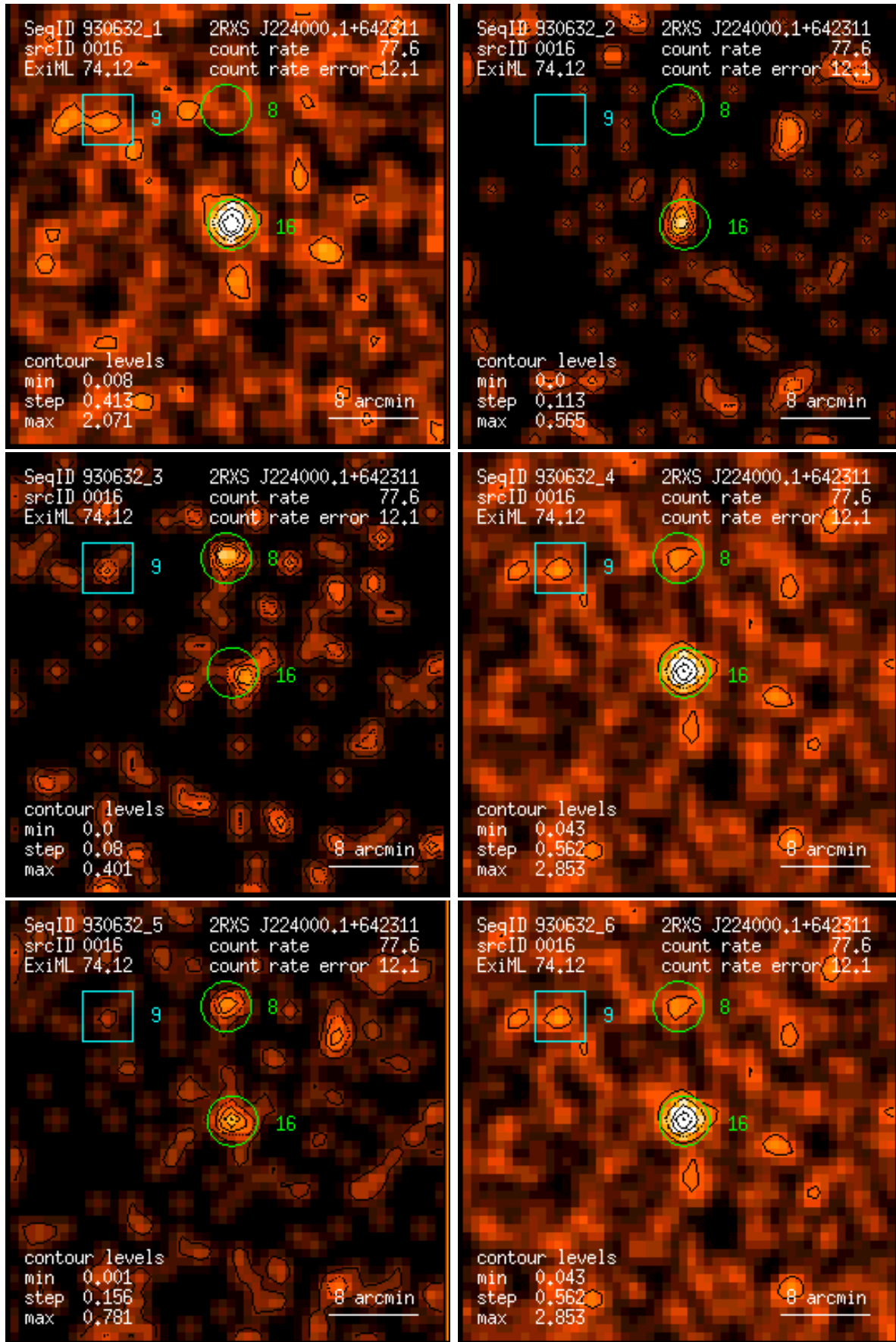
Figure 16: RASS 930632: detection 0016: band rate images, Gaussian filter: (1) PSPC channels 11 – 41, (2) 52 – 90, (3) 91 – 201, (4) 11 – 235, (5) 52 – 201, (6) 11 – 201. Broad band rates in counts/ks. Band rate contour levels in counts/ks/arcmin 2 .
