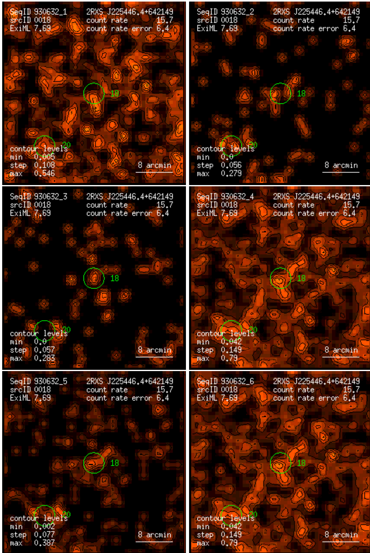
Figure 18: RASS 930632: detection 0018: band rate images, Gaussian filter: (1) PSPC channels 11 – 41, (2) 52 – 90, (3) 91 – 201, (4) 11 – 235, (5) 52 – 201, (6) 11 – 201. Broad band rates in counts/ks. Band rate contour levels in counts/ks/arcmin 2 .
