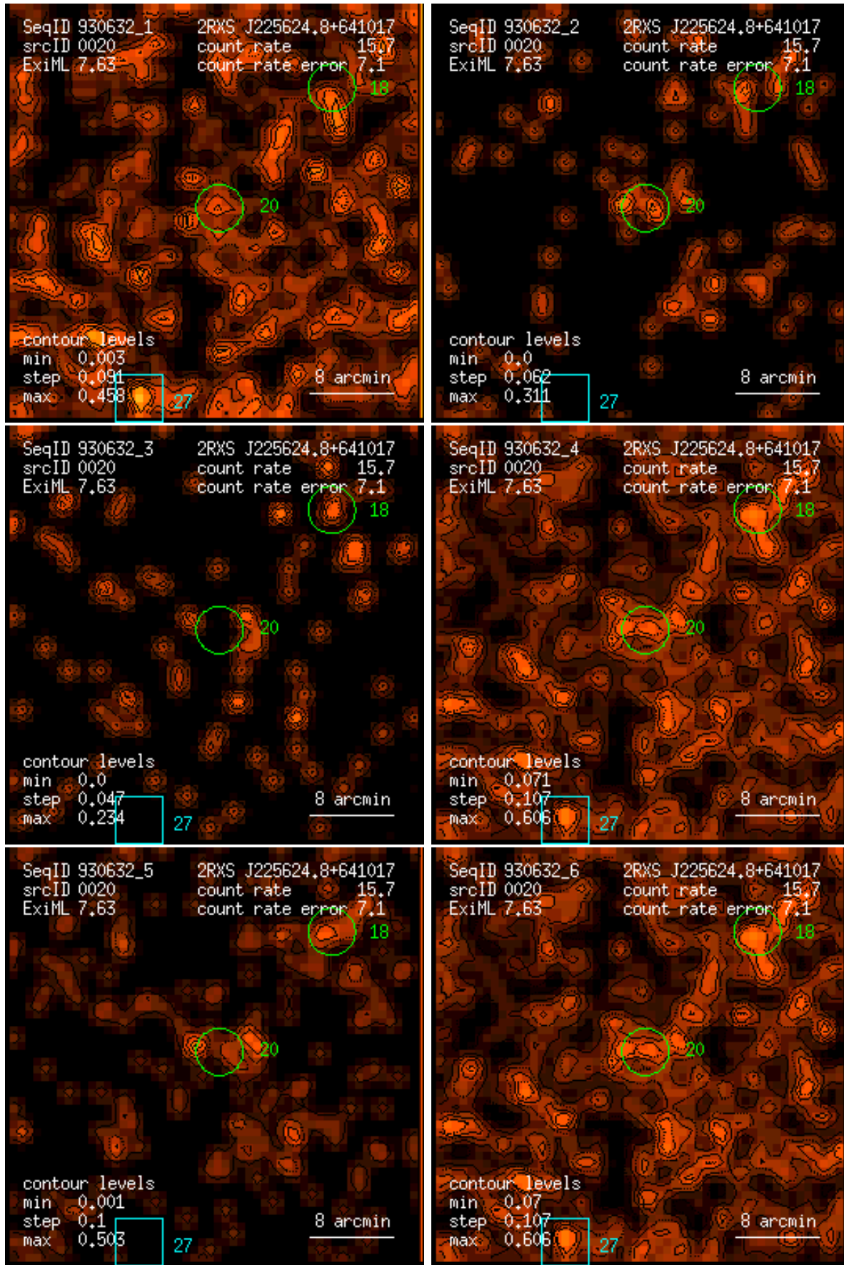
Figure 20: RASS 930632: detection 0020: band rate images, Gaussian filter: (1) PSPC channels 11 – 41, (2) 52 – 90, (3) 91 – 201, (4) 11 – 235, (5) 52 – 201, (6) 11 – 201. Broad band rates in counts/ks. Band rate contour levels in counts/ks/arcmin 2 .
