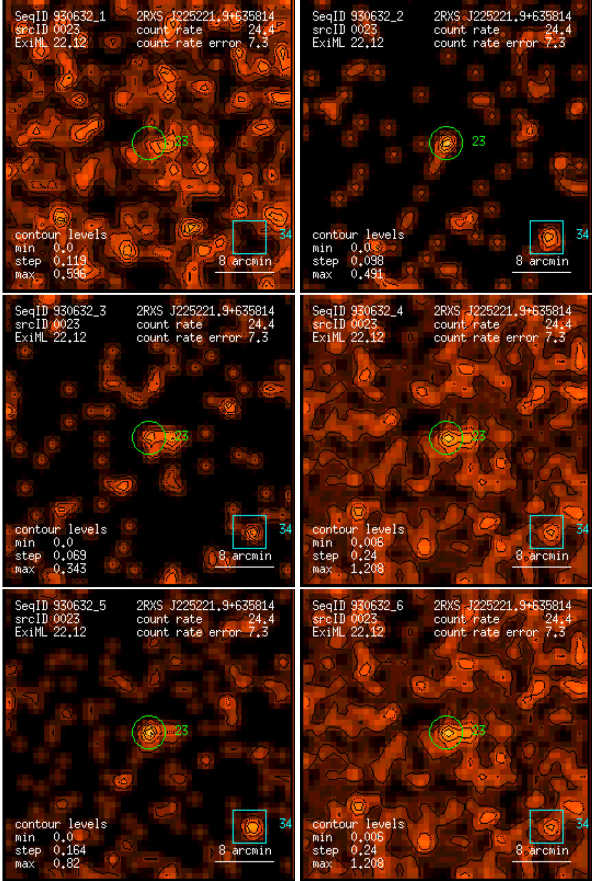
Figure 23: RASS 930632: detection 0023: band rate images, Gaussian filter: (1) PSPC channels 11 – 41, (2) 52 – 90, (3) 91 – 201, (4) 11 – 235, (5) 52 – 201, (6) 11 – 201. Broad band rates in counts/ks. Band rate contour levels in counts/ks/arcmin 2 .
