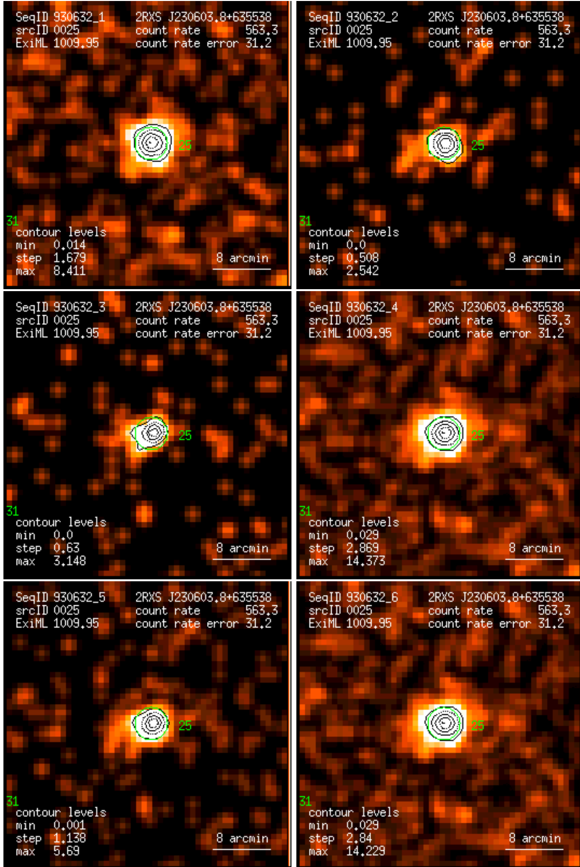
Figure 25: RASS 930632: detection 0025: band rate images, Gaussian filter: (1) PSPC channels 11 – 41, (2) 52 – 90, (3) 91 – 201, (4) 11 – 235, (5) 52 – 201, (6) 11 – 201. Broad band rates in counts/ks. Band rate contour levels in counts/ks/arcmin 2 .
