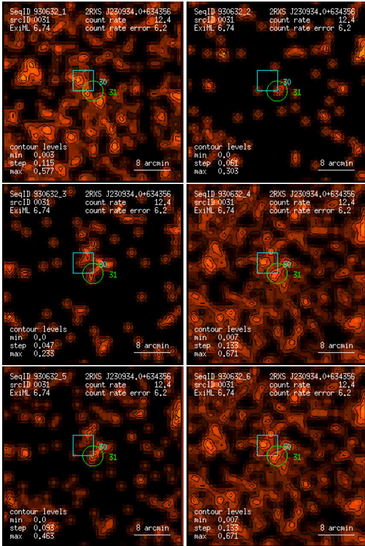
Figure 31: RASS 930632: detection 0031: band rate images, Gaussian filter: (1) PSPC channels 11 – 41, (2) 52 – 90, (3) 91 – 201, (4) 11 – 235, (5) 52 – 201, (6) 11 – 201. Broad band rates in counts/ks. Band rate contour levels in counts/ks/arcmin 2 .
