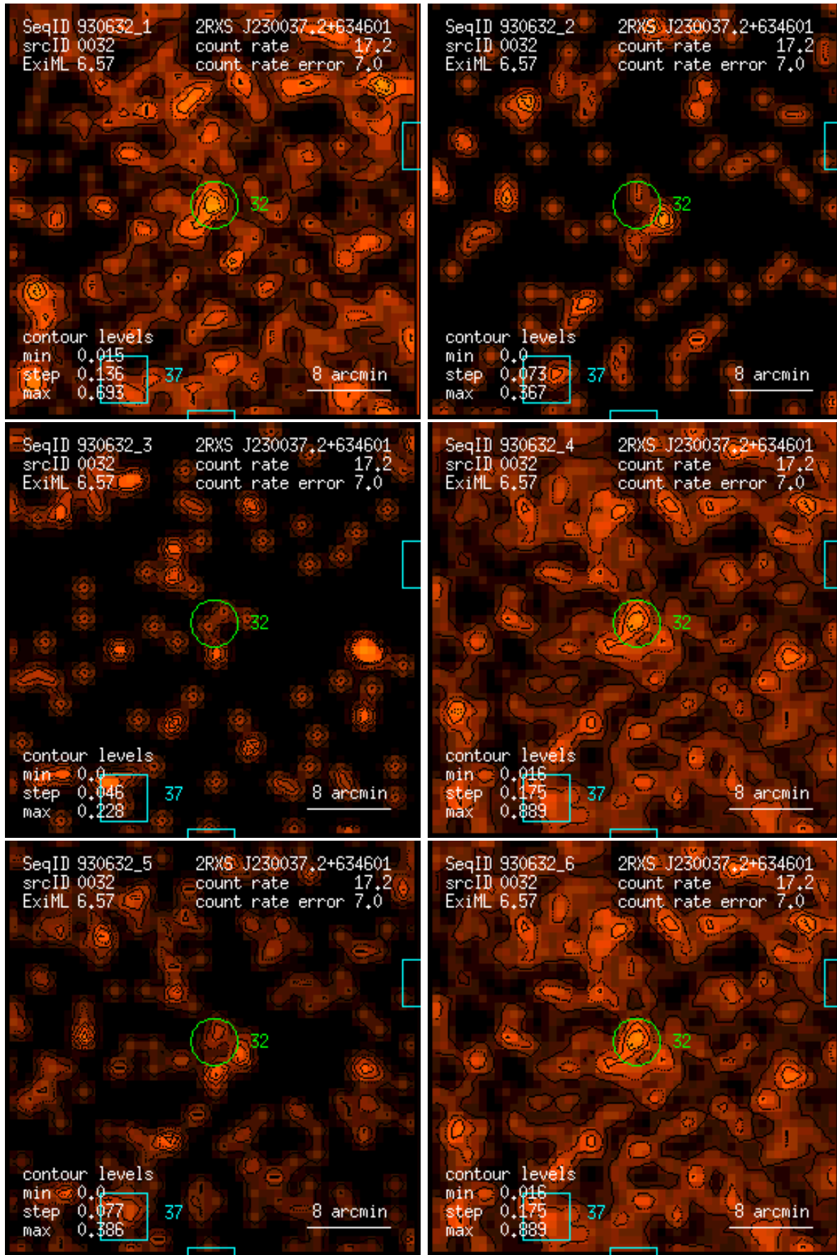
Figure 32: RASS 930632: detection 0032: band rate images, Gaussian filter: (1) PSPC channels 11 – 41, (2) 52 – 90, (3) 91 – 201, (4) 11 – 235, (5) 52 – 201, (6) 11 – 201. Broad band rates in counts/ks. Band rate contour levels in counts/ks/arcmin 2 .
