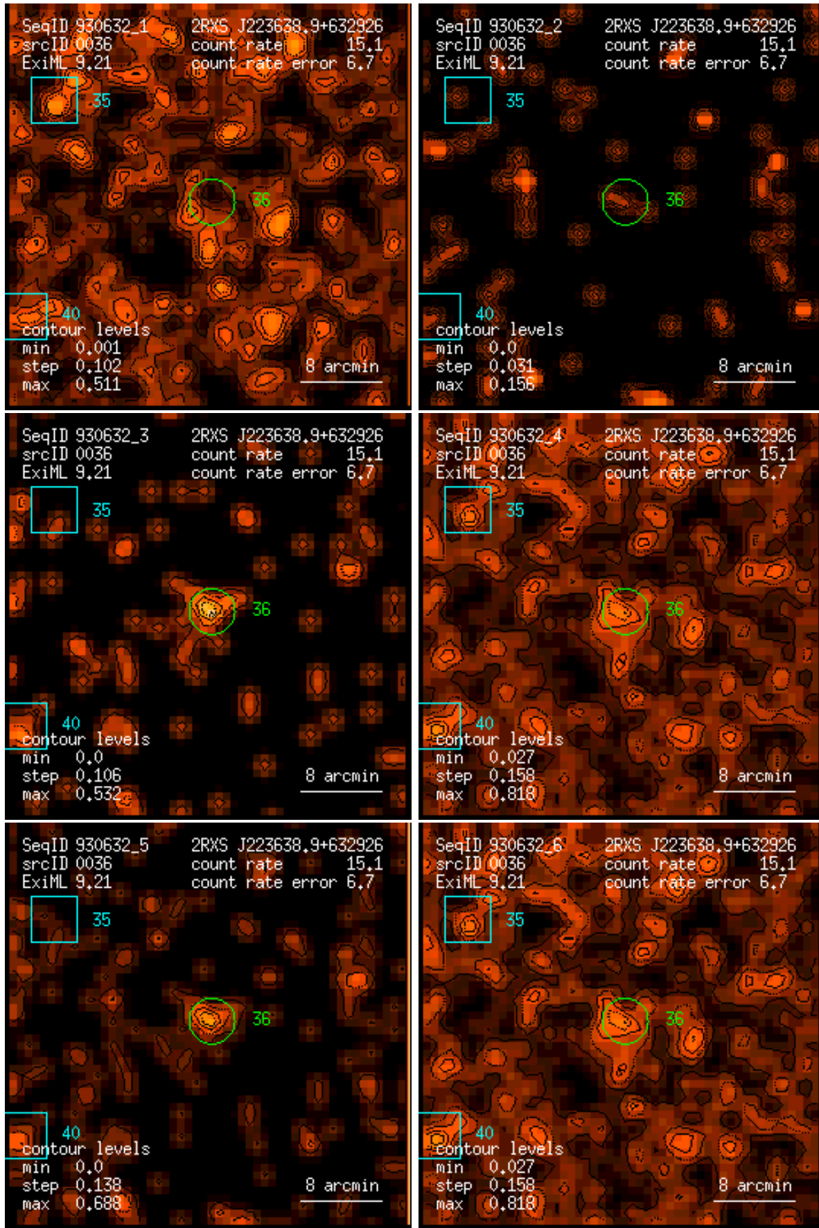
Figure 36: RASS 930632: detection 0036: band rate images, Gaussian filter: (1) PSPC channels 11 – 41, (2) 52 – 90, (3) 91 – 201, (4) 11 – 235, (5) 52 – 201, (6) 11 – 201. Broad band rates in counts/ks. Band rate contour levels in counts/ks/arcmin 2 .
