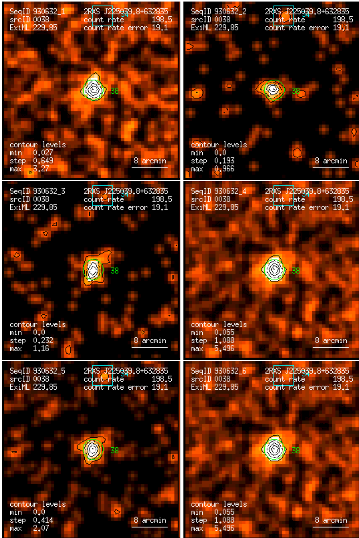
Figure 38: RASS 930632: detection 0038: band rate images, Gaussian filter: (1) PSPC channels 11 – 41, (2) 52 – 90, (3) 91 – 201, (4) 11 – 235, (5) 52 – 201, (6) 11 – 201. Broad band rates in counts/ks. Band rate contour levels in counts/ks/arcmin 2 .
